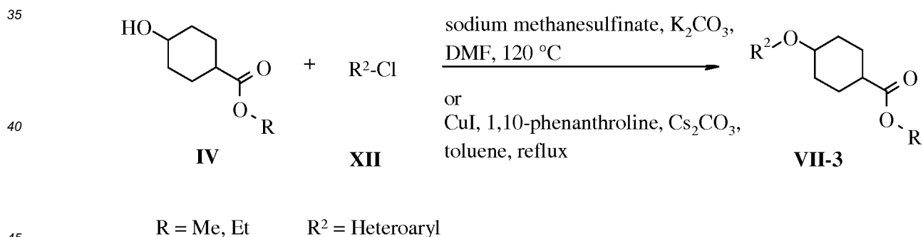
Scheme 6: General Scheme F
