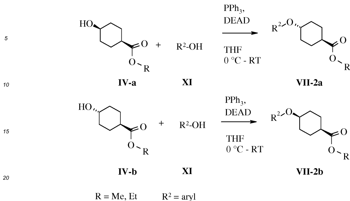
Scheme 5: General Scheme E
