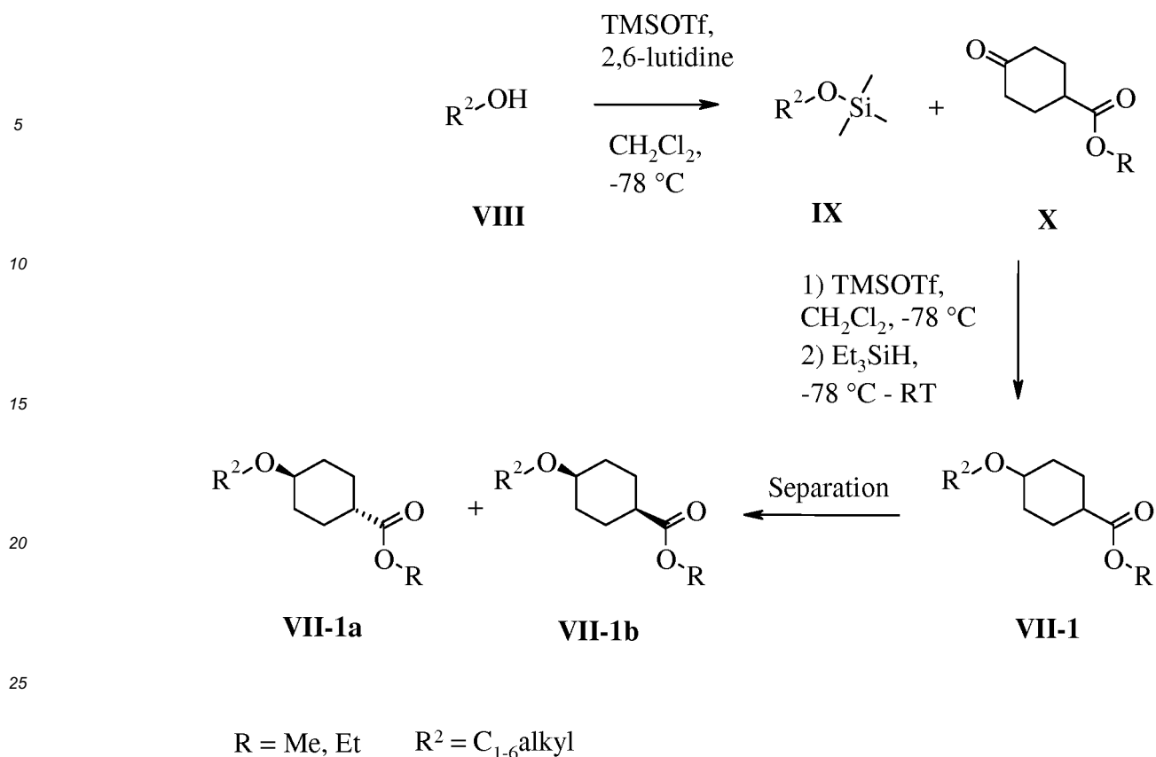
Scheme 4: General Scheme D
