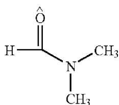
N,N-dimethylformamide
