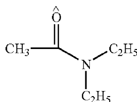
N,N-diethylacetamide
