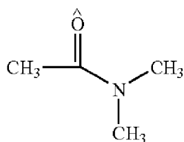
N,N-dimethylacetamide
