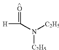
N,N-diethylformamide
