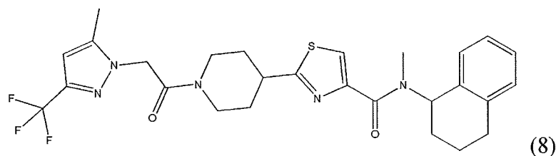
[Chem. 9]
