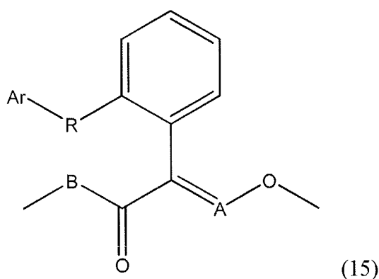
[Chem. 15]
