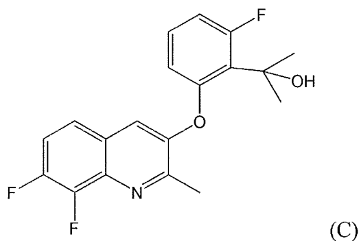
[Chem. 22]
