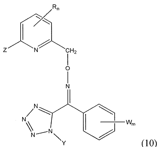
[Chem. 10]
