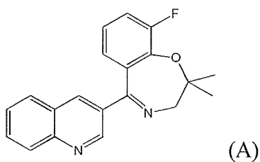
[Chem. 20]
