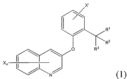
[Chem. 1]
