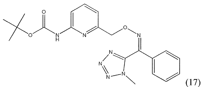
[Chem. 17]
