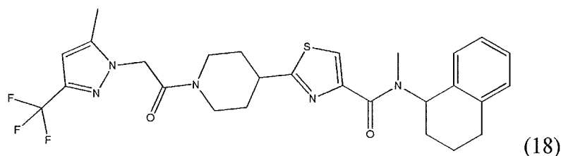
[Chem. 19]
