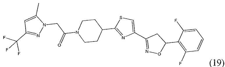
[Chem. 19]
