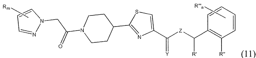
[Chem. 11]
