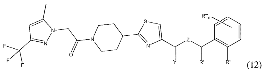
[Chem. 12]
