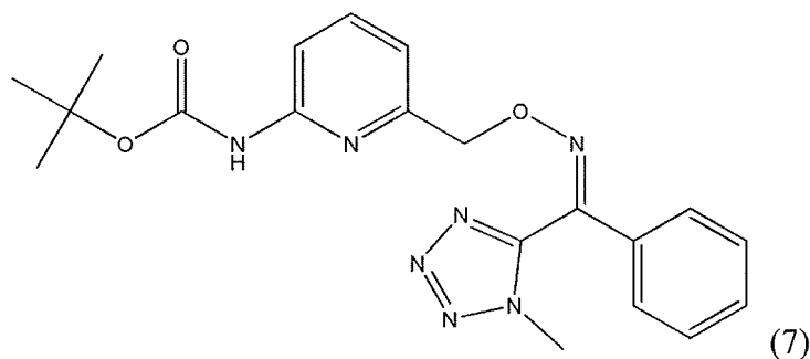
[Chem. 7]
