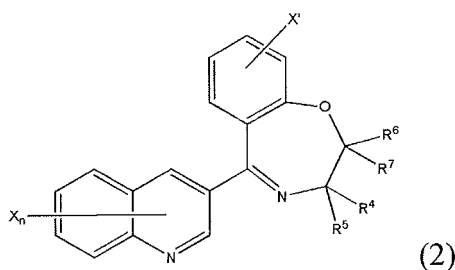
[Chem. 2]
