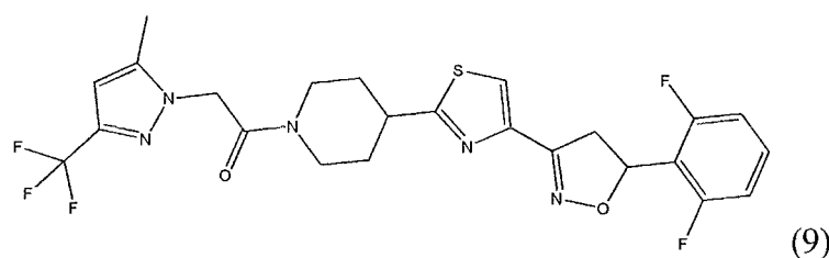
[Chem. 9]
