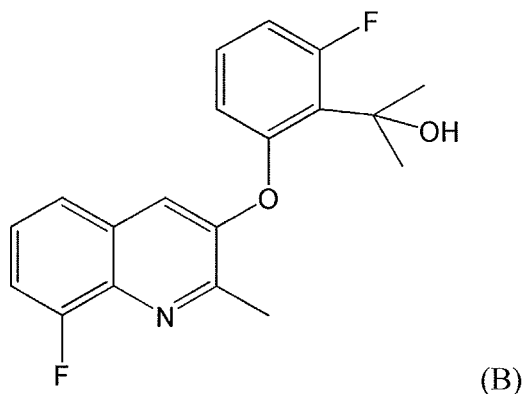
[Chem. 22]
