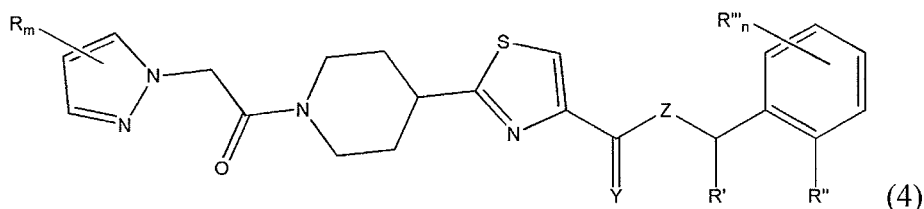
[Chem. 4]
