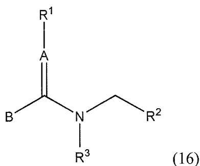
[Chem. 16]
