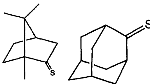
[Chem. 20]
