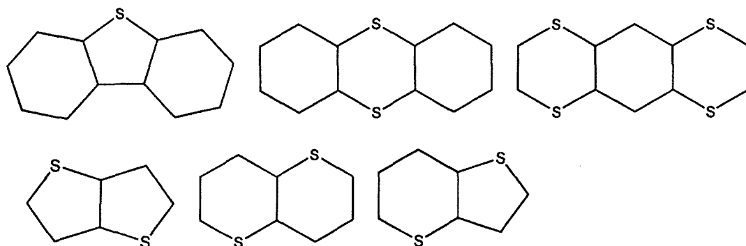
[Chem. 39]
