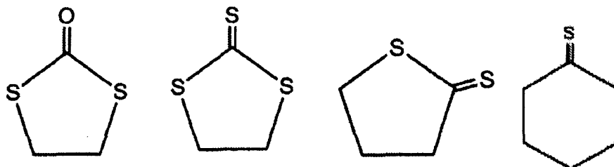
[Chem. 19]
