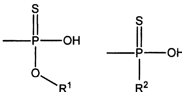
[Chem. 15]
