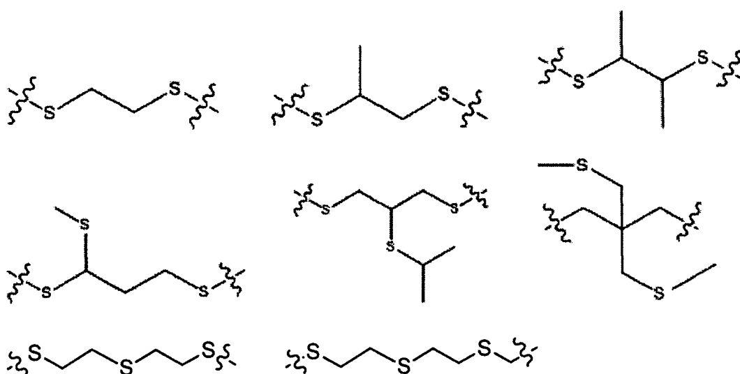
[Chem. 44]
