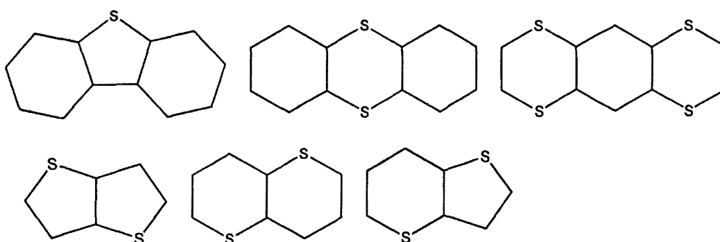
[Chem. 21]
