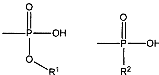
[Chem. 14]
