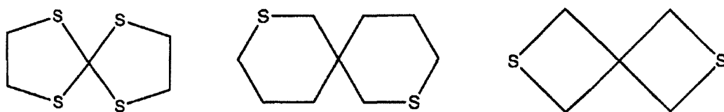
[Chem. 40]
