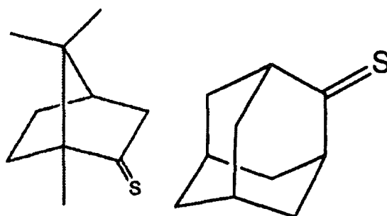
[Chem. 38]
