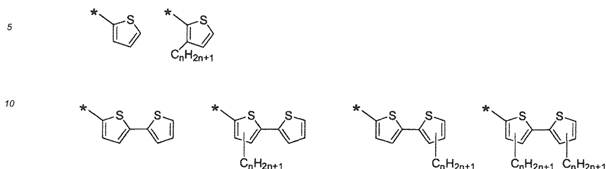
[Chemical Formula 30]
