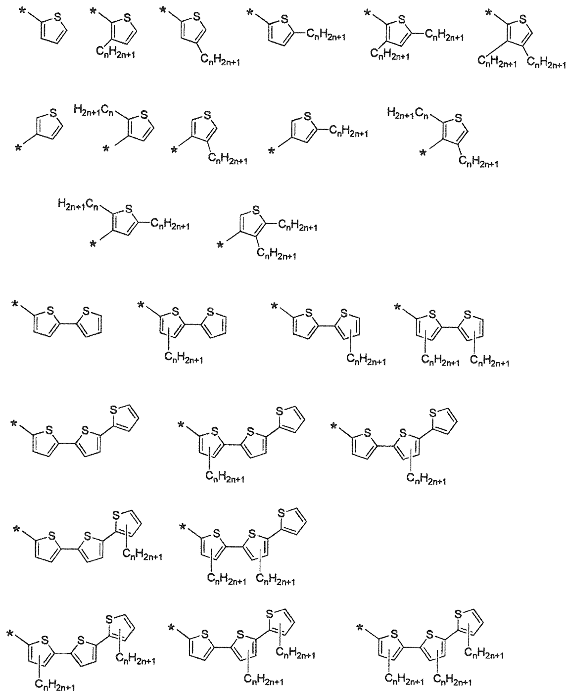
[Chemical Formula 27]
