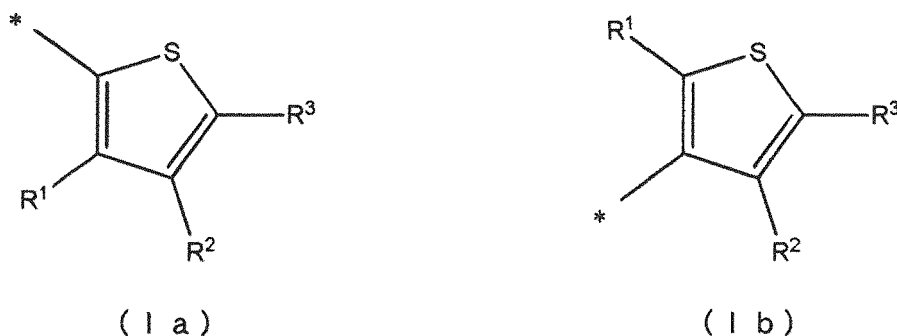
[Chemical Formula 22]
