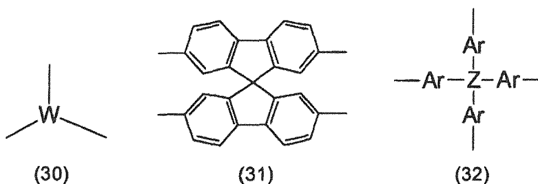
[Chemical Formula 21]
