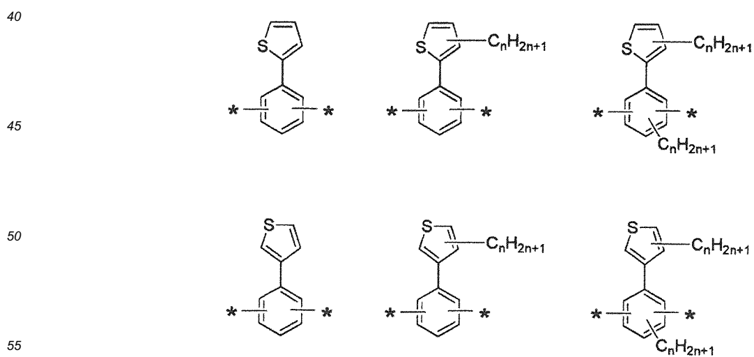
[Chemical Formula 29]
