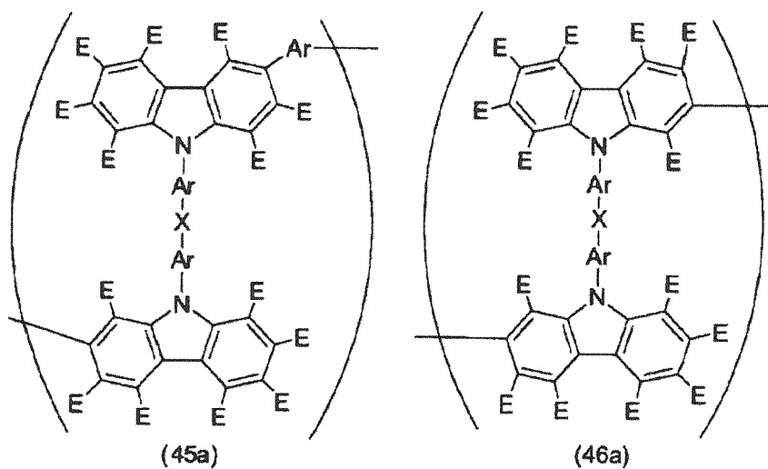
[Chemical Formula 6]
