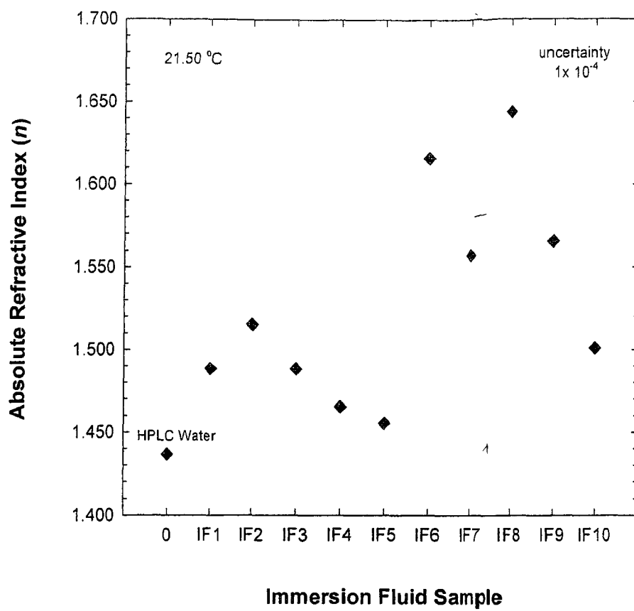
Figure 4. Absolute Refractive index of Immersion Fluids @ 193nm
