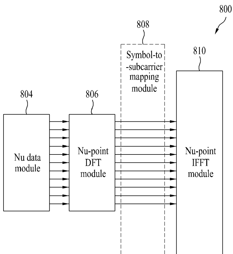
Localized DFT-s-OFDMA
