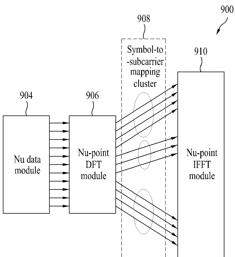
Clusters DFT-s-OFDMA
