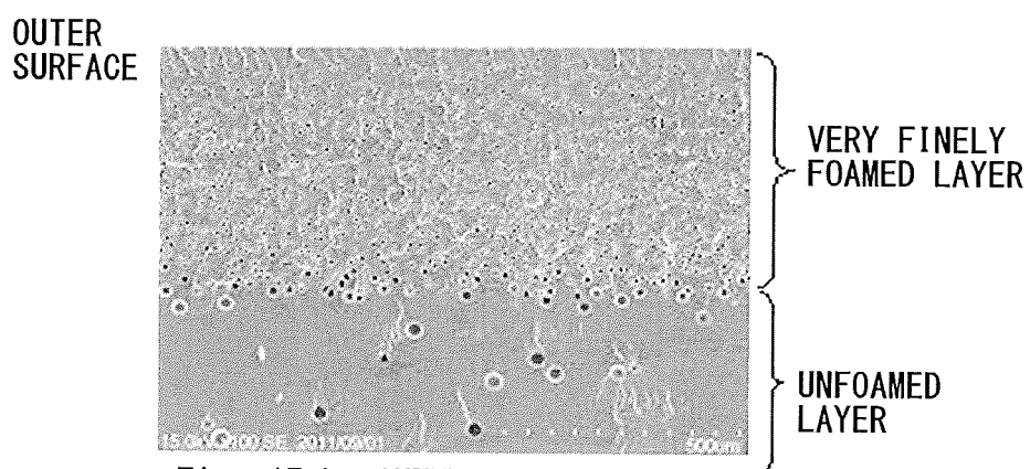
Fig. 17-b: OUTER SURFACE SIDE ON AN ENLARGED SCALE
