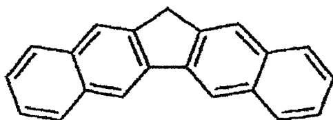
[Chem. 9]
