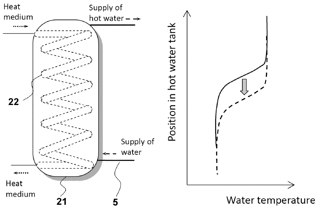
Conceptual diagram of variation in water temperature in hot water tank
