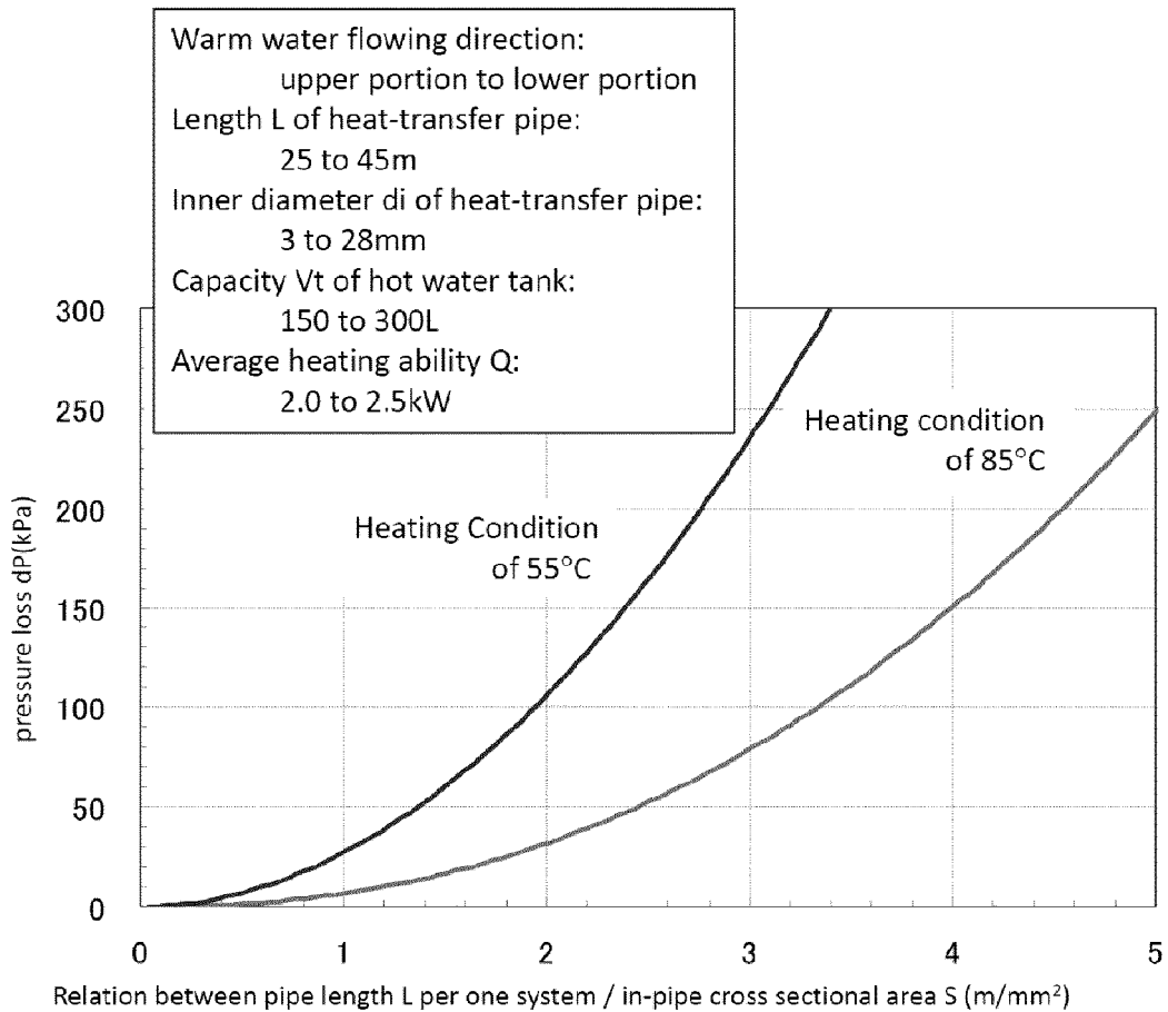
Diagram showing relation between pressure loss dP when hot water is stored and pile length L / in-pipe cross sectional area S
