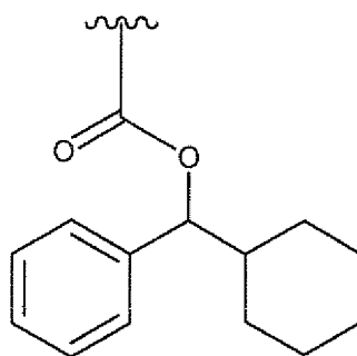
[Chemical Formula 15]
