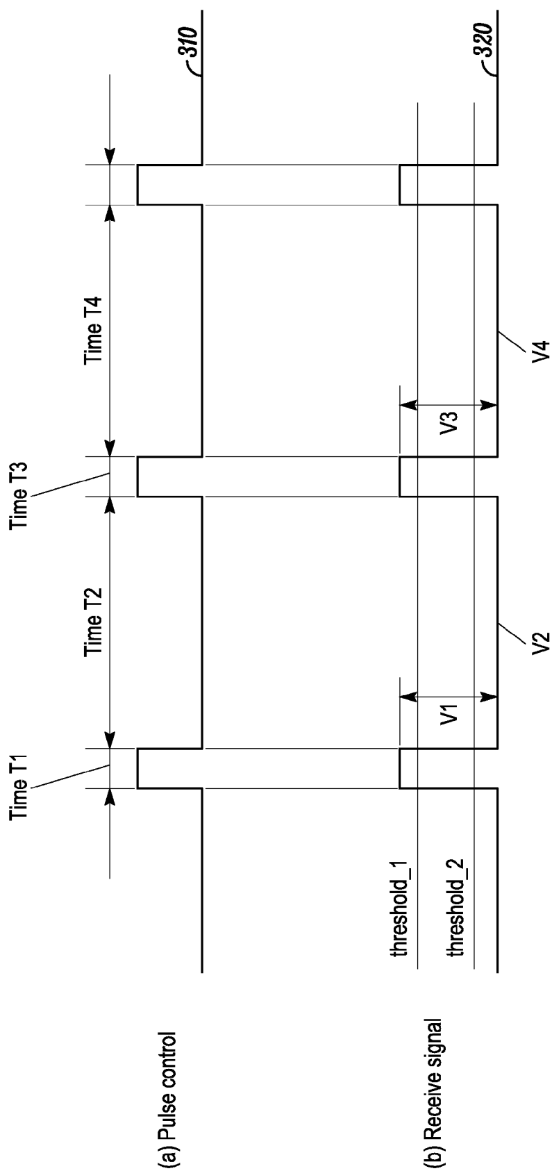
An embodiment control wave of IR receiving
