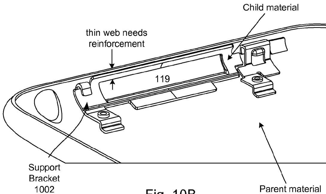
Fig. 10B After punching operation with dock opening formed
