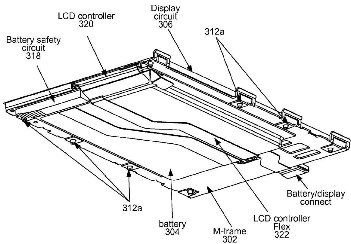
Fig. 2D M frame (assembled)
