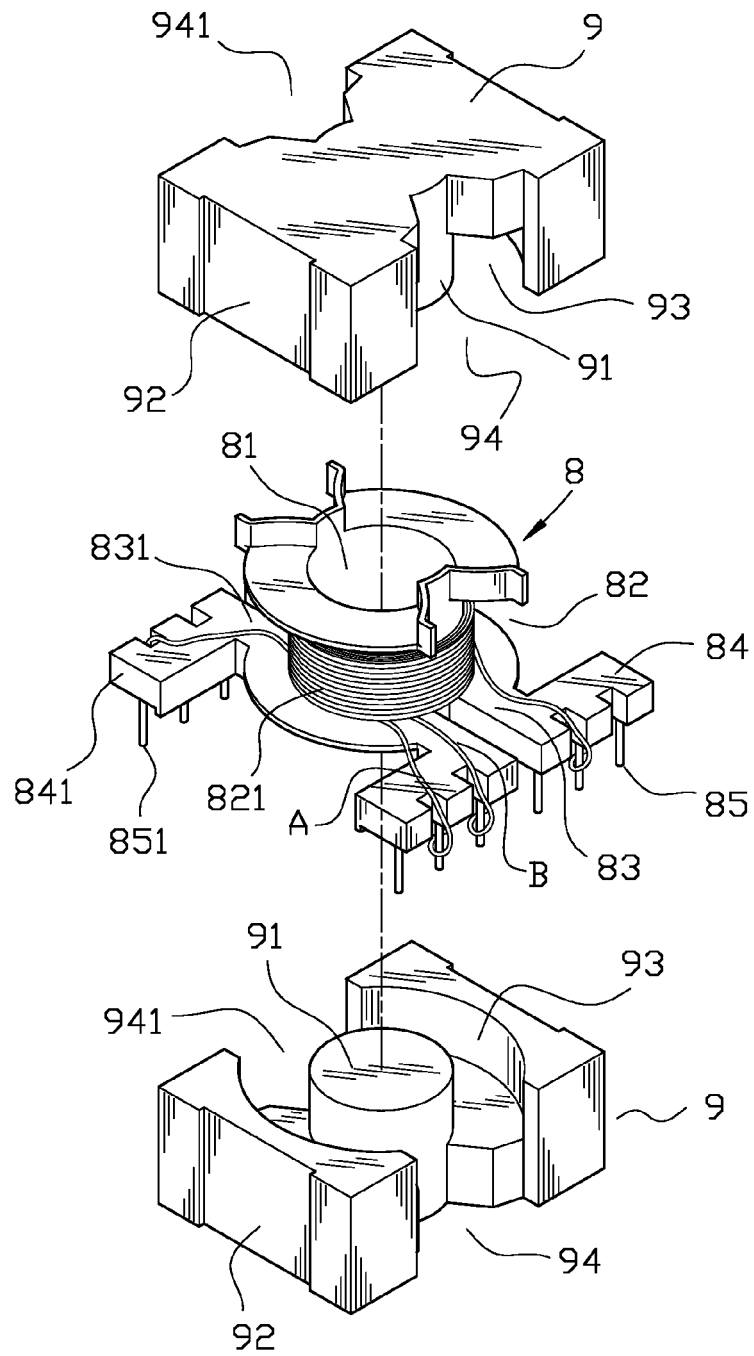
Fig.1 (Prior Art)
