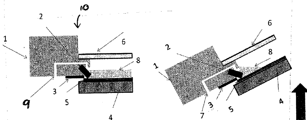
Fig 2. a) Horizontal cell with fluid outlet path 7. b) tilted cell with small volume of electrolyte.
