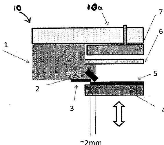
Figure 1. Schematic cross section of chamber edge.
