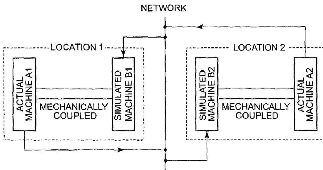
FIG. 1 RELATED ART
