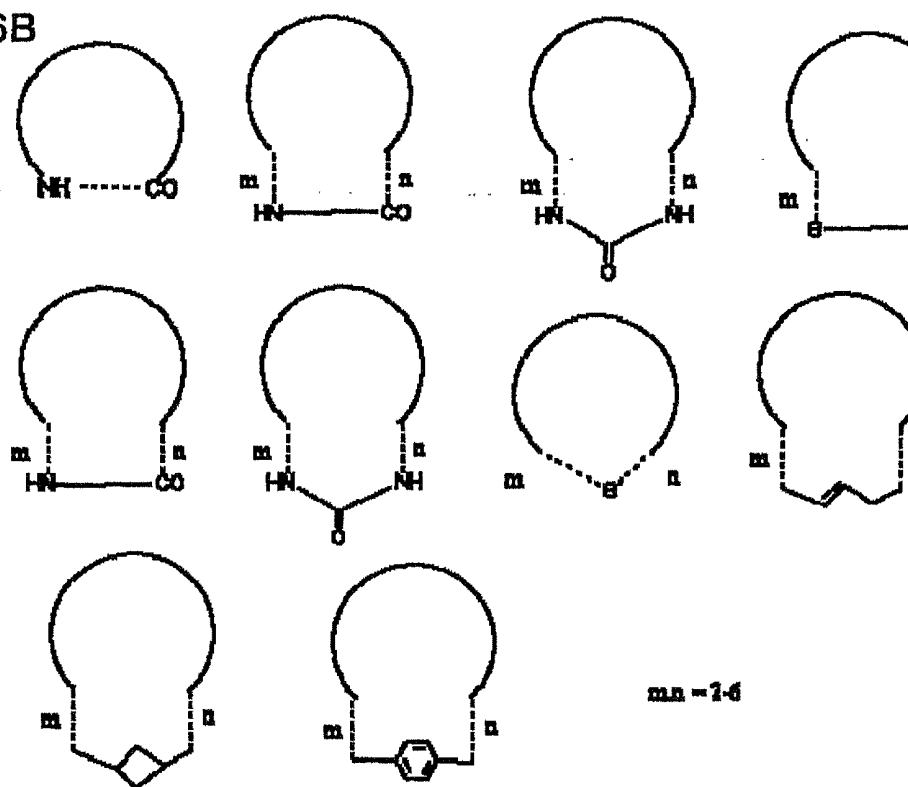
Scheme 2. Cyclization strategies:
