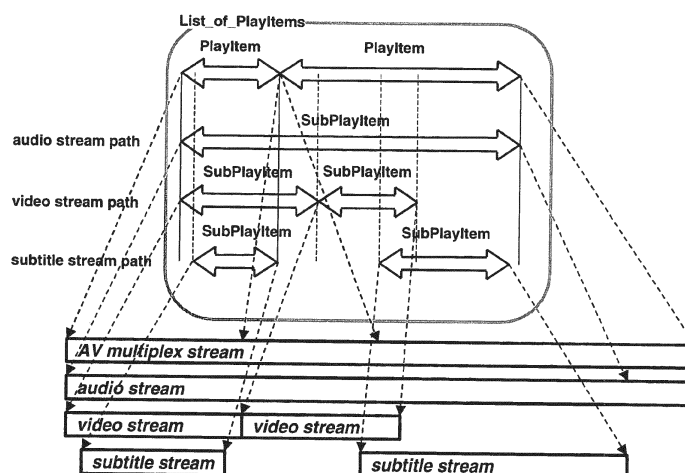
Figure 1: List_of_PlayItems Example
