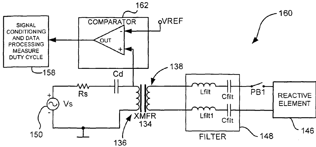
VOLTAGE/CURRENT SOURCE WITH DUTY CYCLE MEASUREMENT
