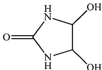
4,5-dihydroxyimidazolidin-2-one
