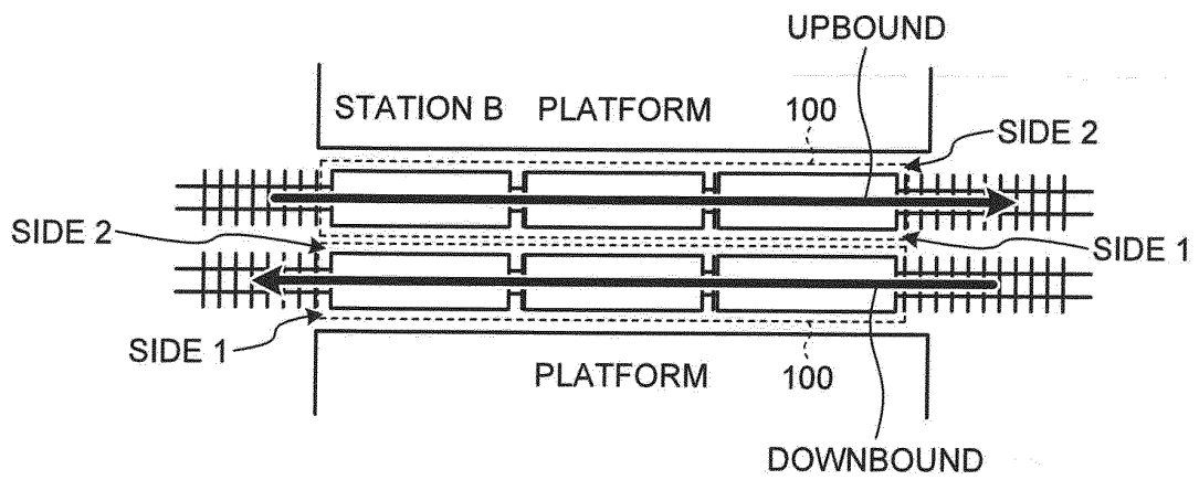
(b) SEPARATE PLATFORMS
