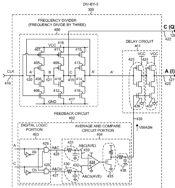
FEEDBACK CONTROLS DELAY CIRCUIT SUCH THAT A IS 90 DEGREES OUT OF PHASE WITH RESPECT TO C
