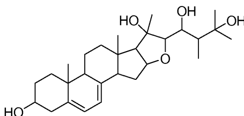
Formula II.
