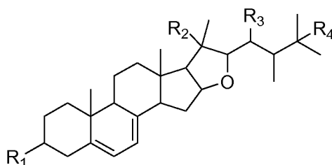
Formula I
