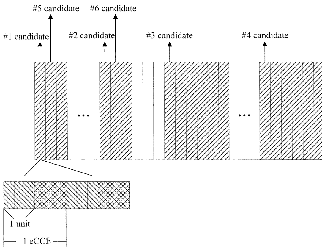
FIG.4/13
