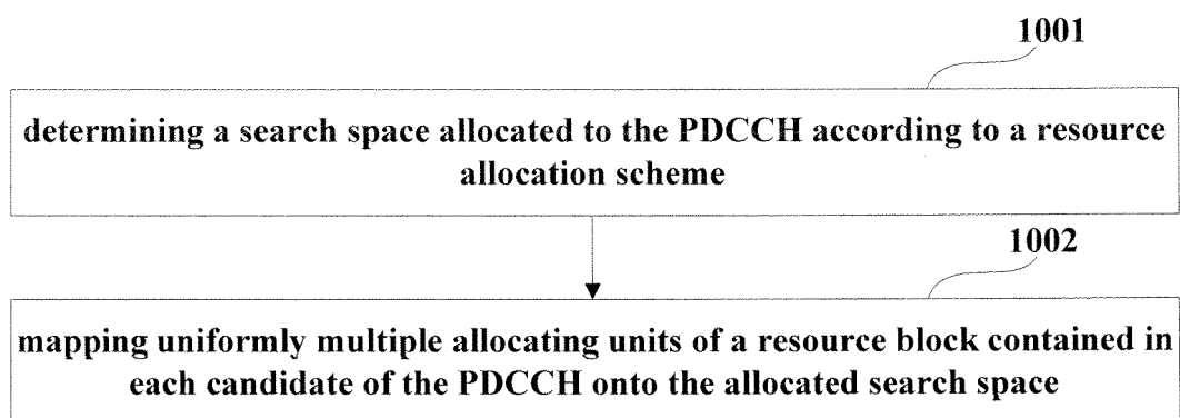
FIG.10/13
