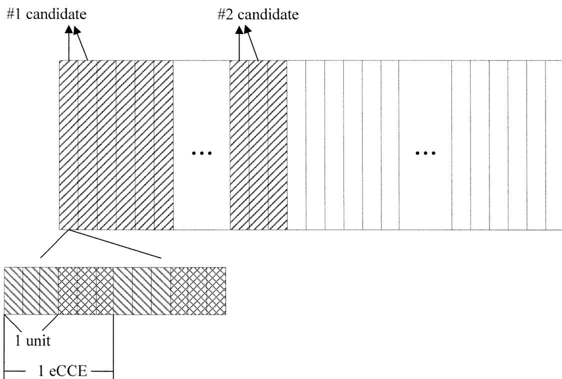
FIG.6/13
