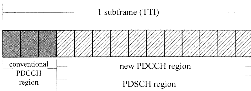
FIG.2/13
