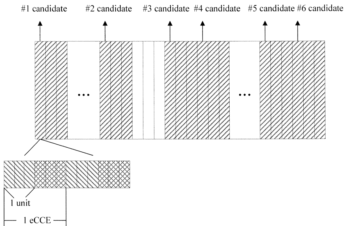
FIG.3/13
