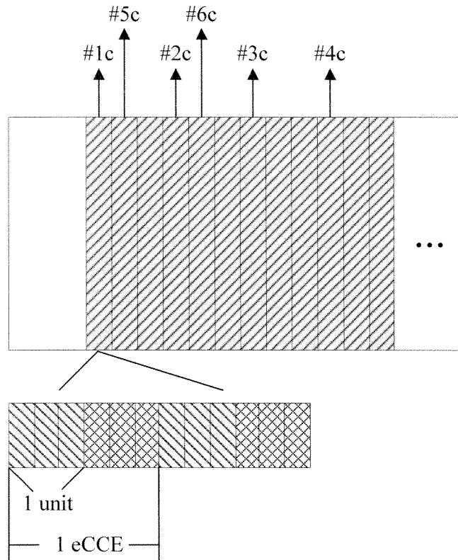
FIG.8/13
