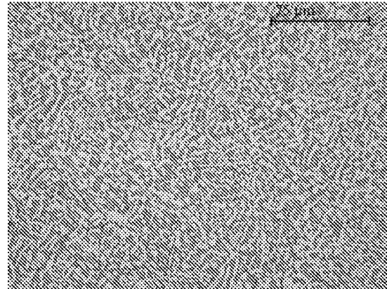
Ti 6Al-2.6V-1Mo (Alloy B)
