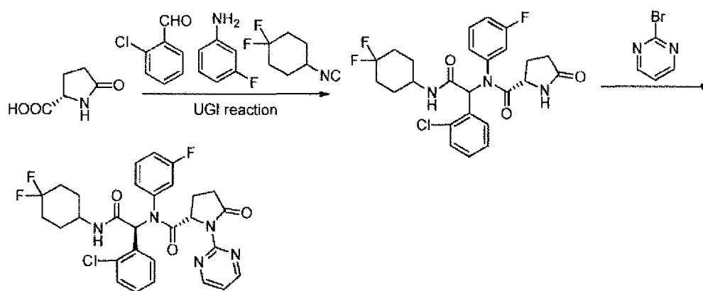
Compound 4
