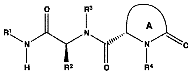
formula II
