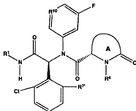
formula II-b
