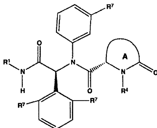
formula II-a-1
