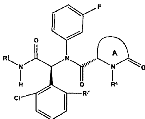
formula II-b-1
