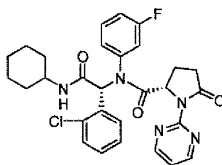
Compound 6
