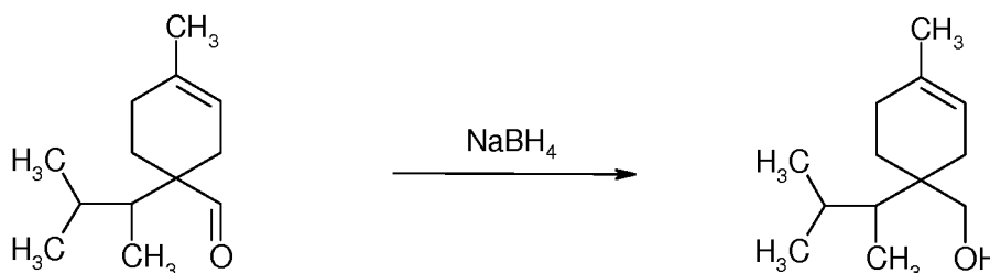
1-(1,2-dimethyl-propyl)-4-methyl-cyclohex-3-enecarbaldehyde
