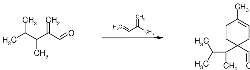
1-(1,2-dimethyl-propyl)-4-methyl-cyclohex-3-enecarbaldehyde
