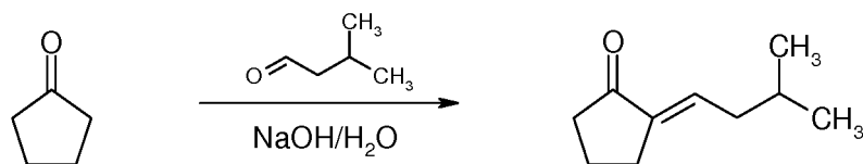
2-[3-methyl-butylidene] -cyclopentanone
