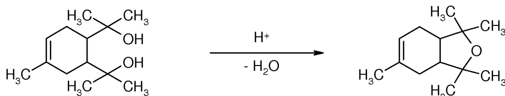
2-[6-(1-hydroxy-1-methyl-ethyl)-4-methyl-cyclohex-3-enyl]-propan-2-ol
