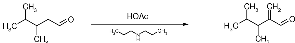
3,4-dimethyl-pentanal
