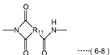
[Chemical formula 29]
