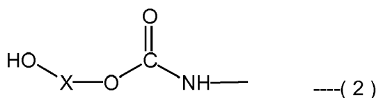
[Chemical formula 6]
