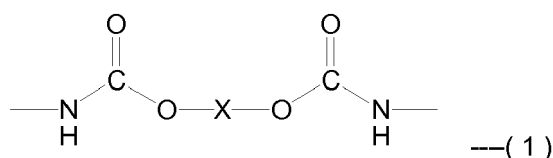
[Chemical formula 6]
