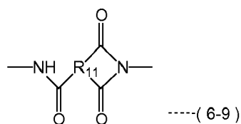
[Chemical formula 29]
