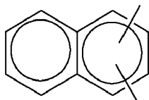
[Chemical formula 14]
