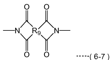
[Chemical formula 28]
