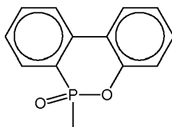
[Chemical formula 12]
