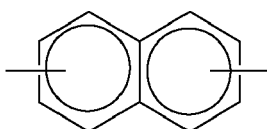
[Chemical formula 14]
