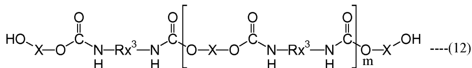
[Chemical formula 18]
