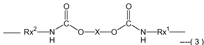
[Chemical formula 7]
