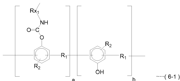
[Chemical formula 17]
