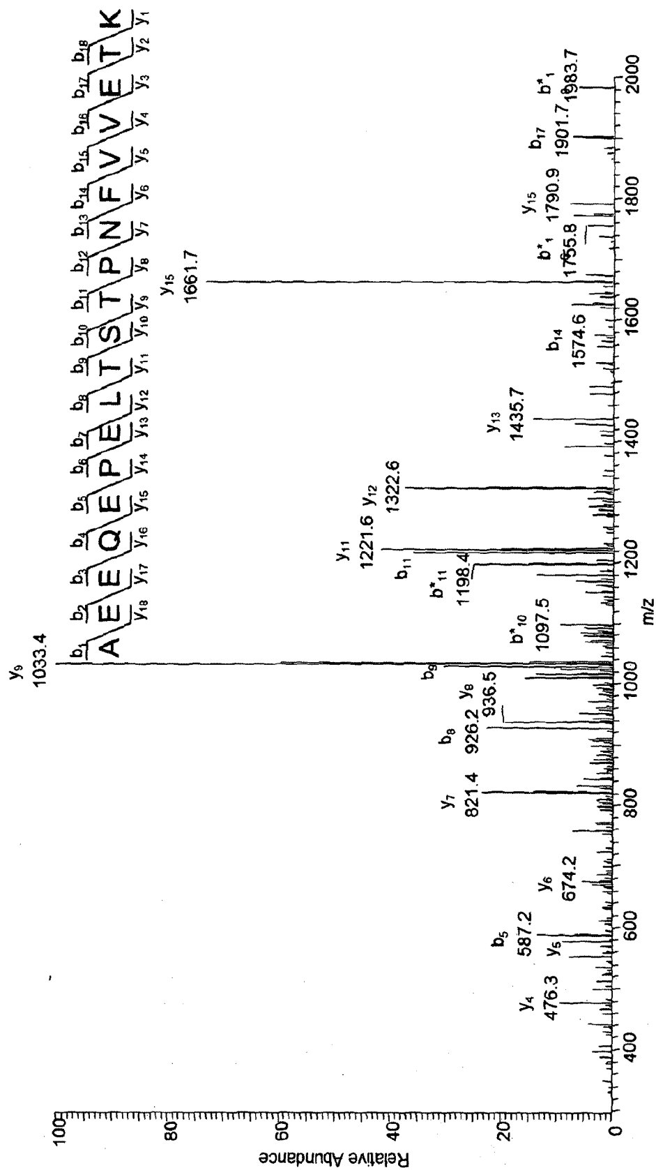
Figure 3C(c) Mass Spectrum for peptide AEEQPELTSTPNFVETK
