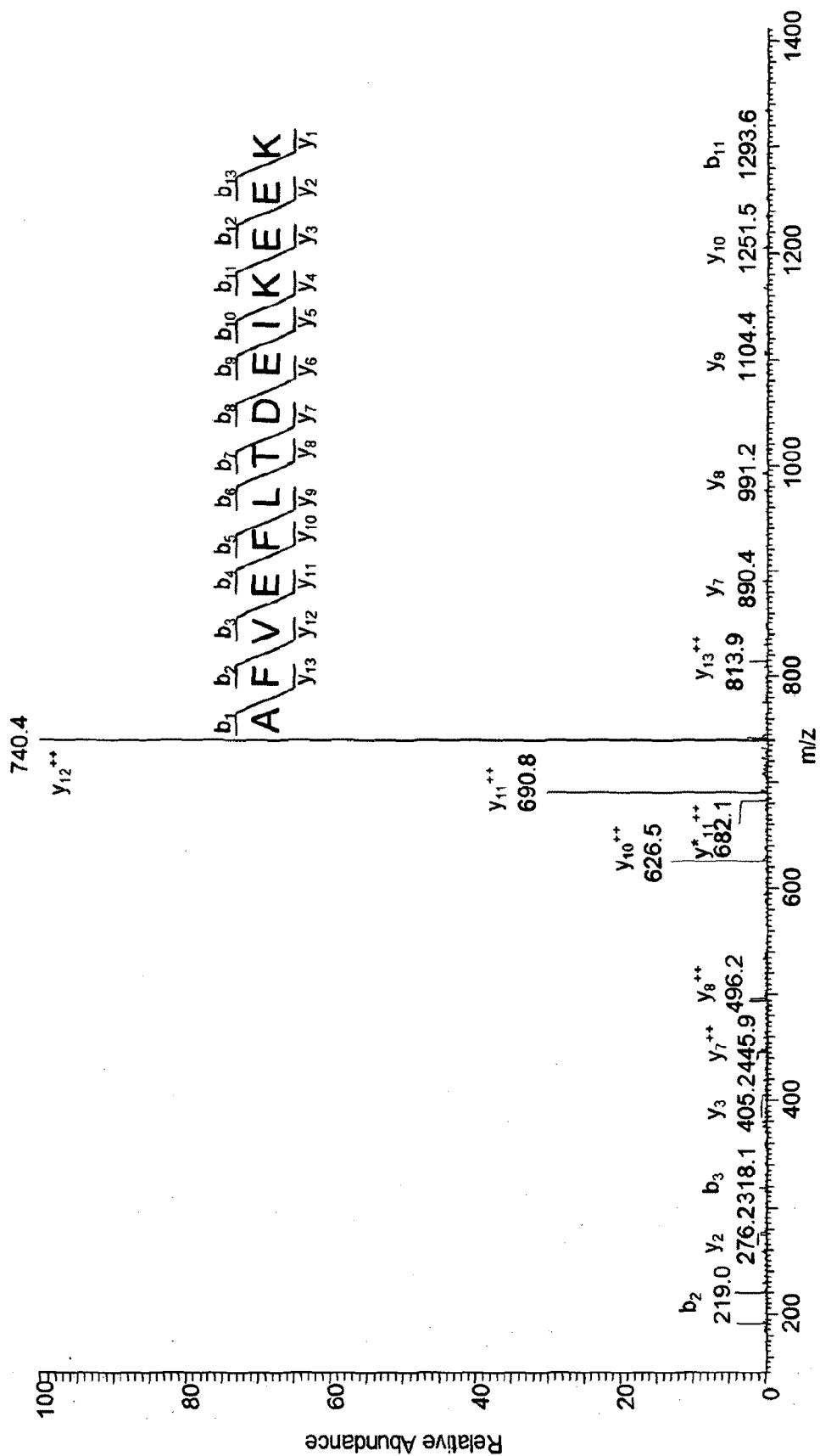
Figure 3C(a) Mass Spectrum for peptide AFVEFLTDEIKEEK
