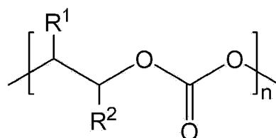
[Chemical Formula 1]
