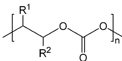
[Chemical Formula 1]
