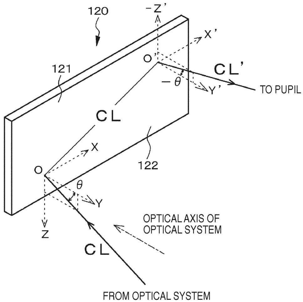
FIG. 28A (EMBODIMENT 15)
