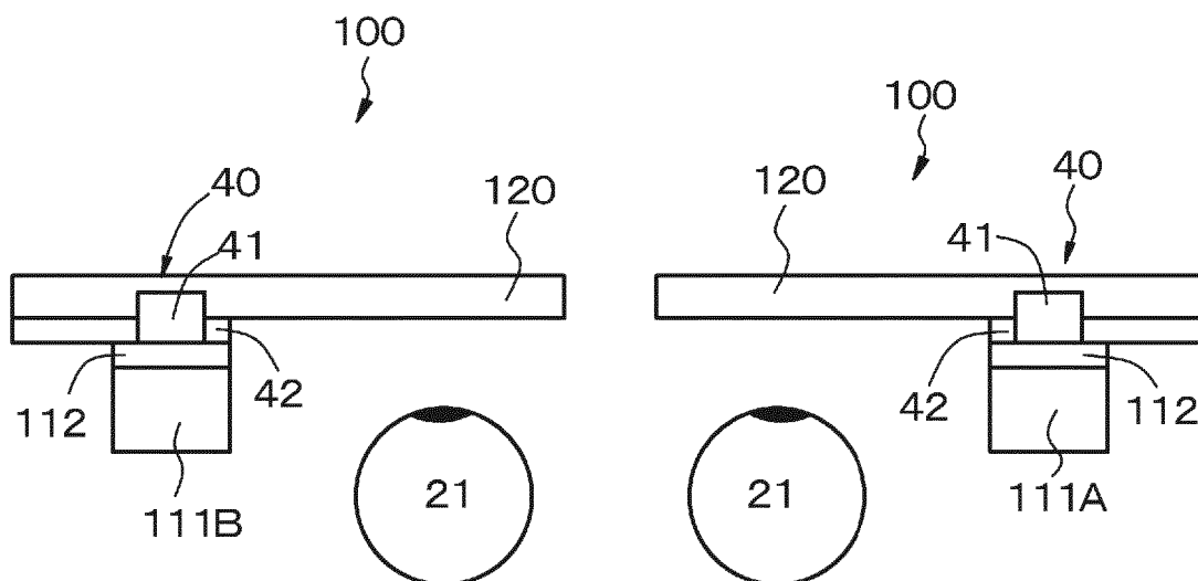
FIG. 35A (EMBODIMENT 20)
