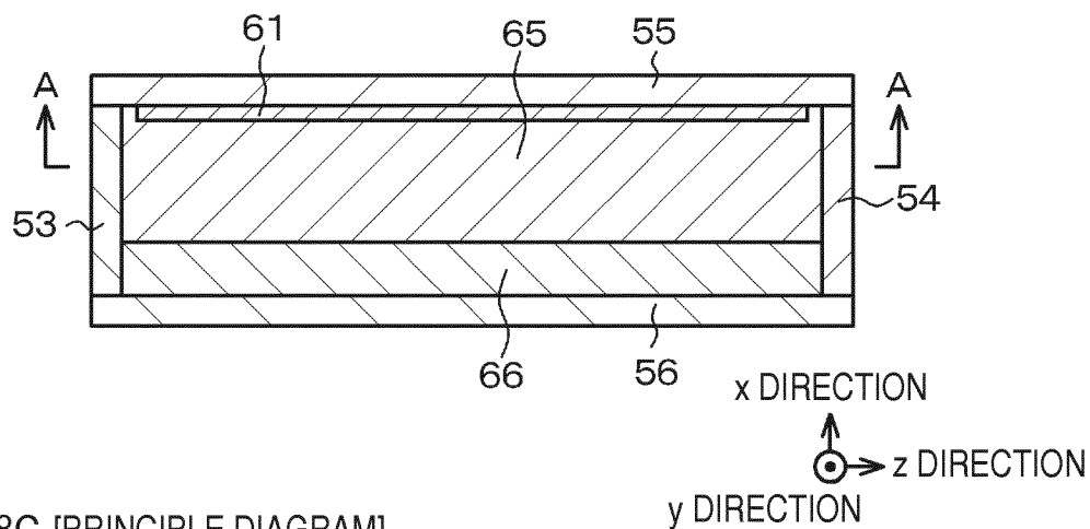
FIG. 38C [PRINCIPLE DIAGRAM]
