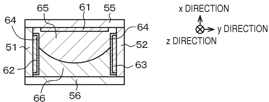
FIG. 38C [PRINCIPLE DIAGRAM]
