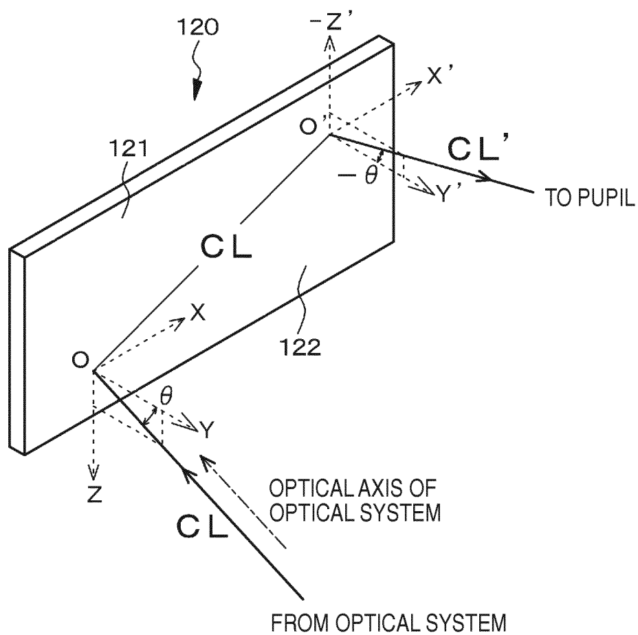
FIG. 26A (EMBODIMENT 14)
