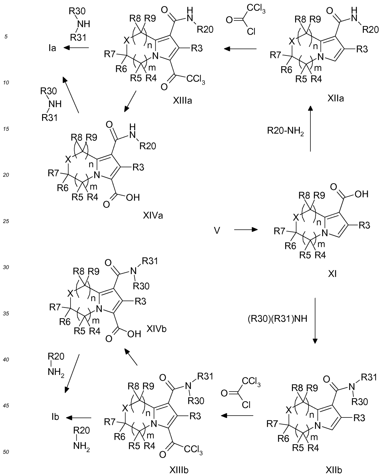
Scheme 6
