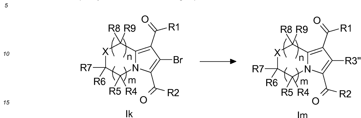
Scheme 13
