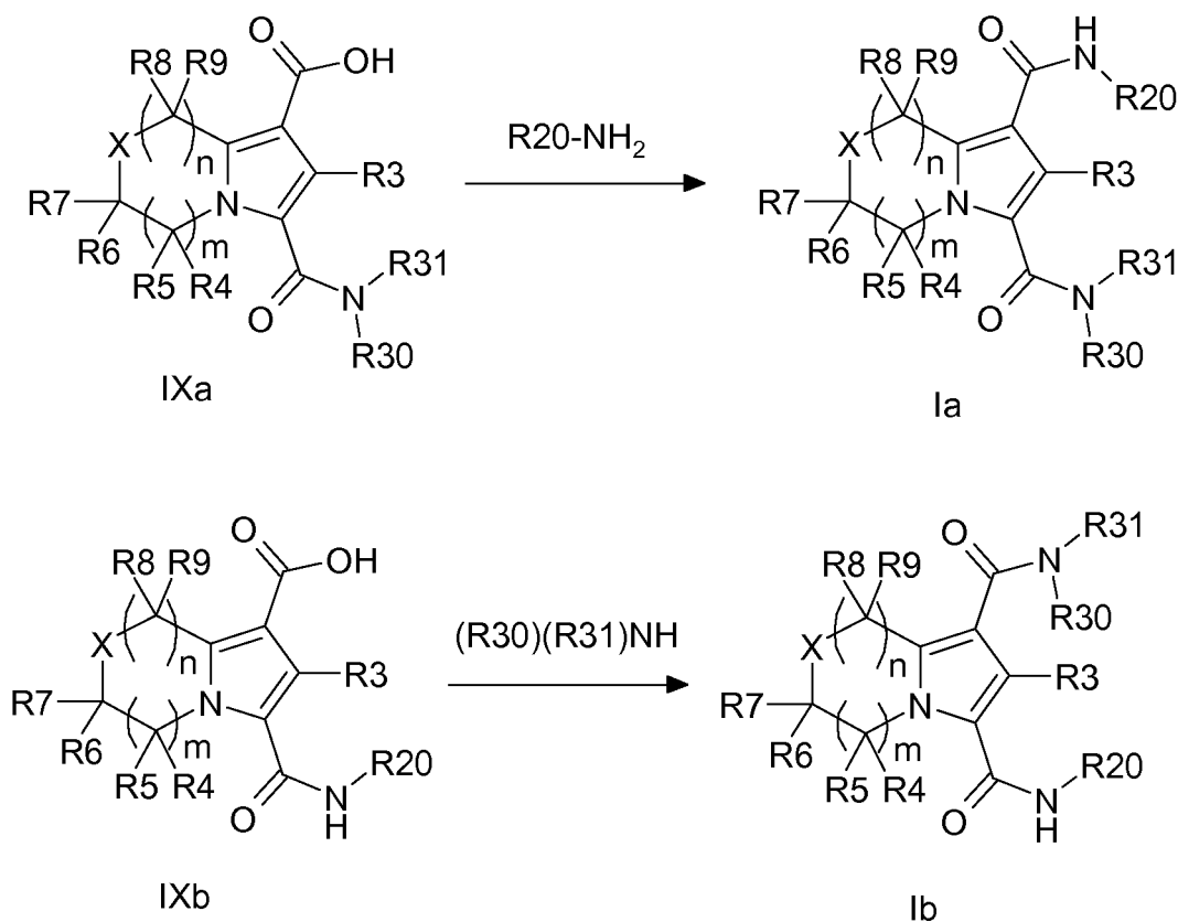
Scheme 5
