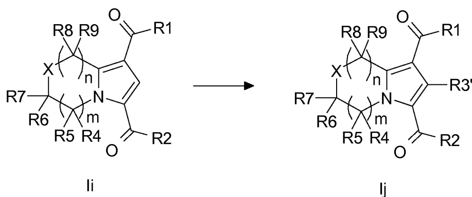
Scheme 12
