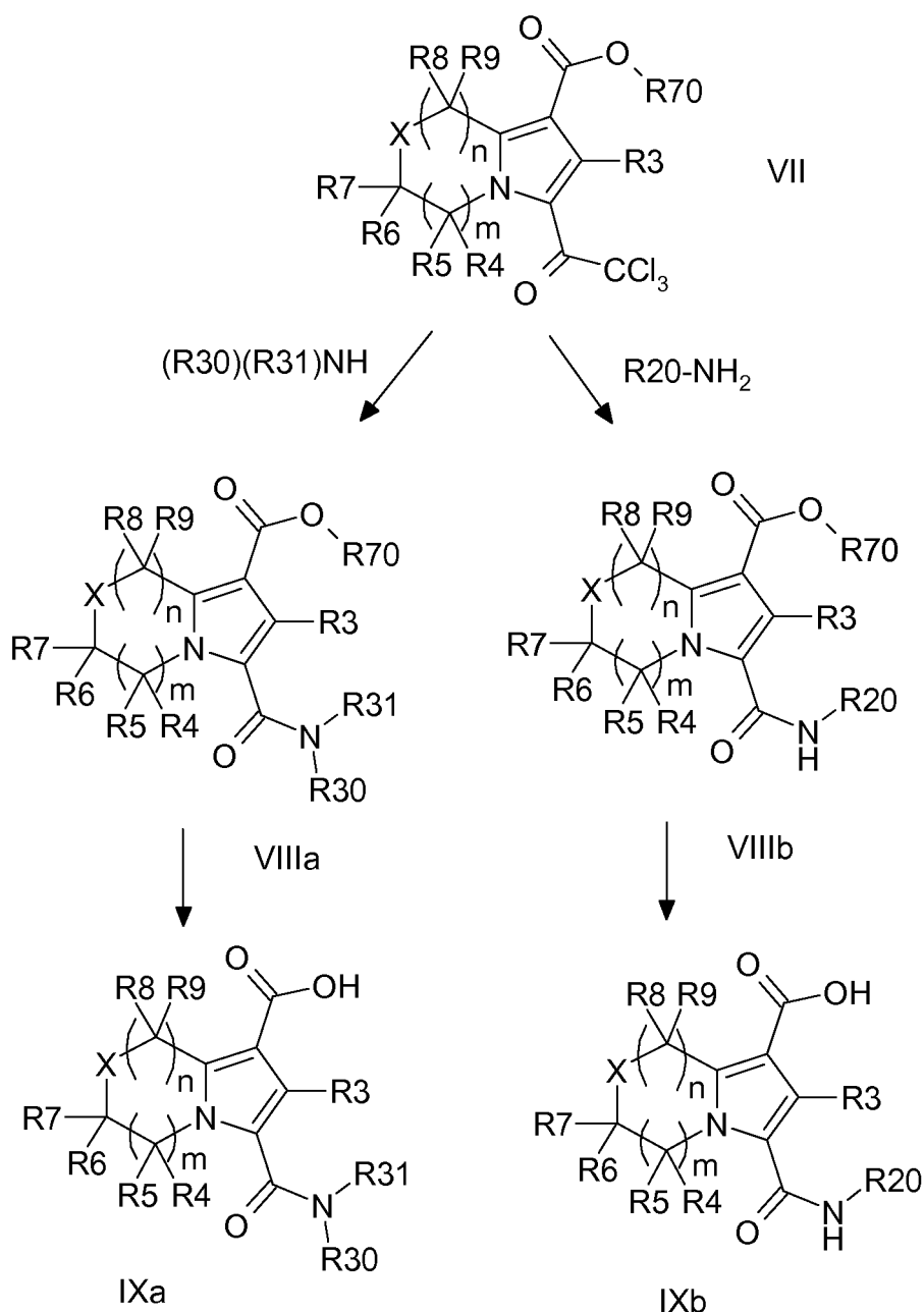
Scheme 3
