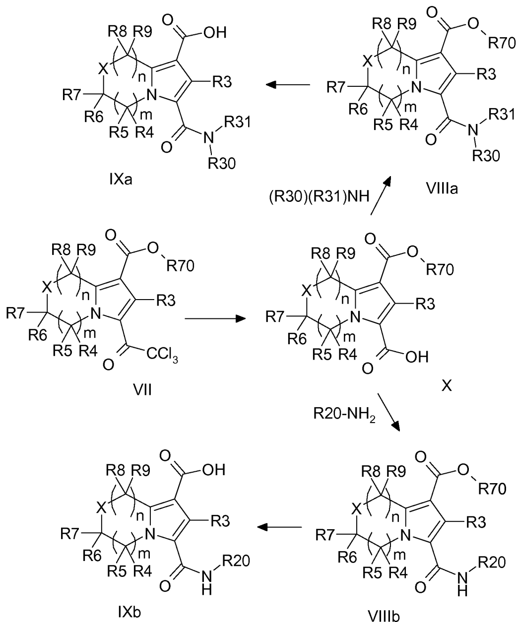
Scheme 4
