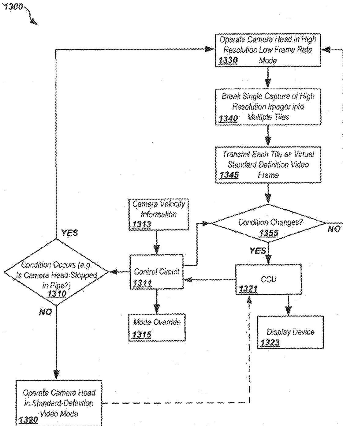
FIG. 13 Example Embodiment of High-Resolution, Low Frame Rate Video Mode Operation
