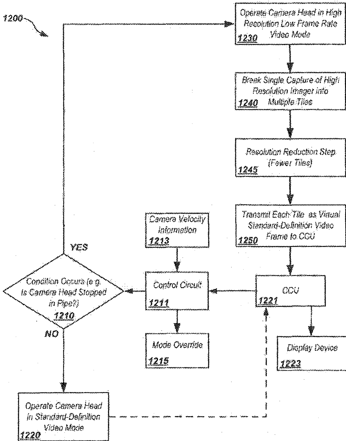
FIG. 12 Example Embodiment of Intermediate-Resolution Still Mode Operation
