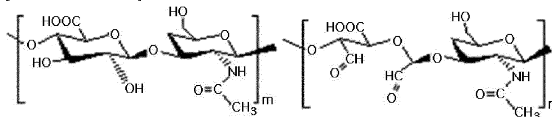
[Chemical formula 1]
