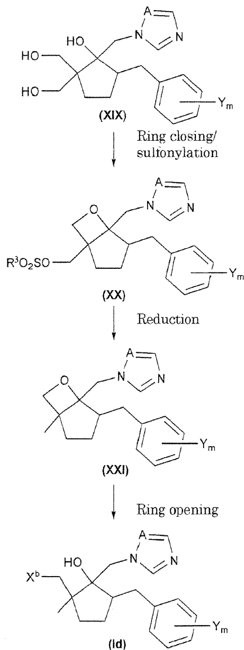
Scheme (10) [Chem.25]
