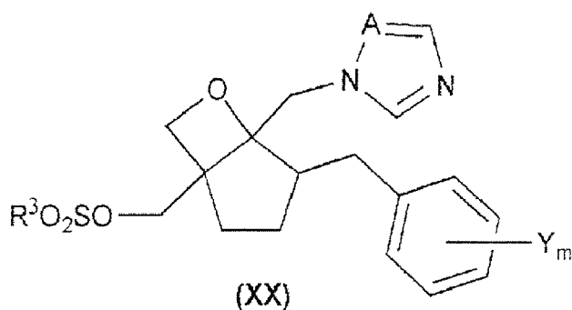
[Chem.13-B]
