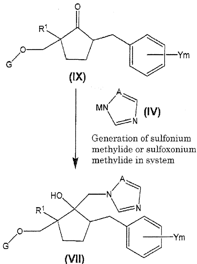
Scheme (4)
