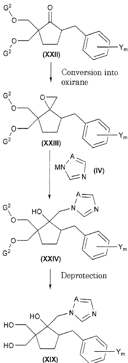
[Chem.26]
