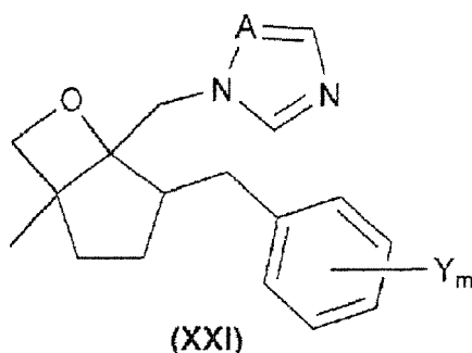
[Chem.13-B]
