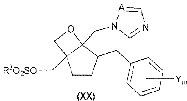
[Chem.13-A]
