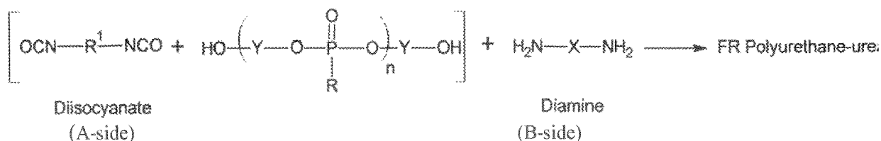
Scheme 1. Preparation of polyurethane-urea coatings
