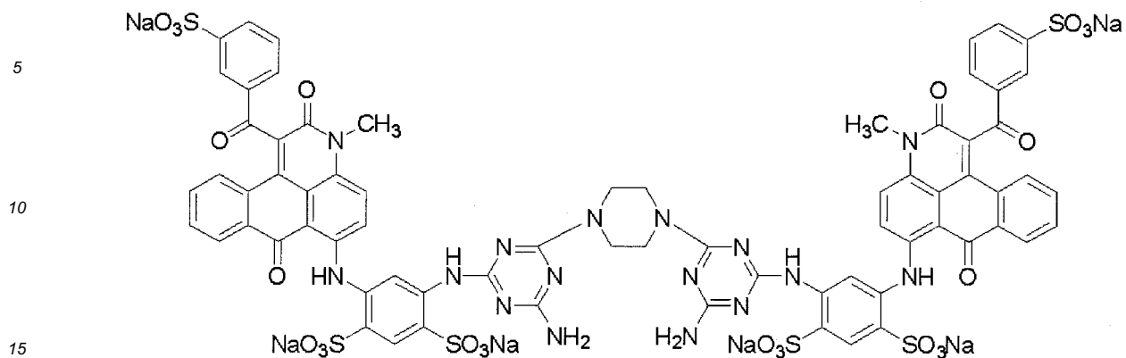
Compound (B3-1)
