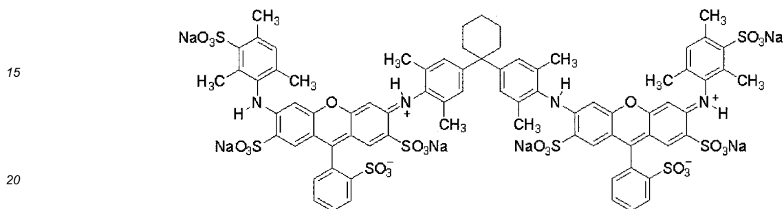
[0160] Exemplary Compound 1-16:
