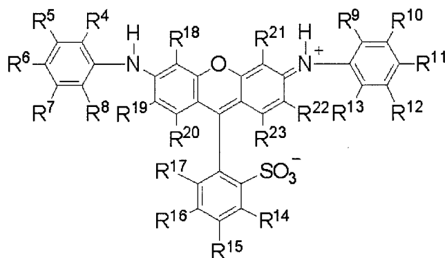
Formula (3)
