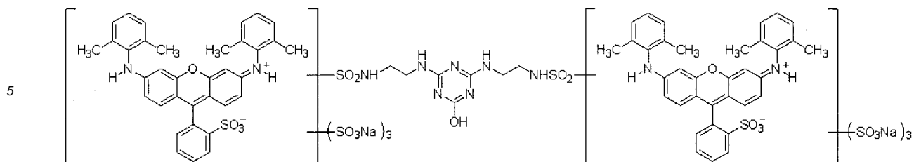
[0159] Exemplary Compound 1-15:
