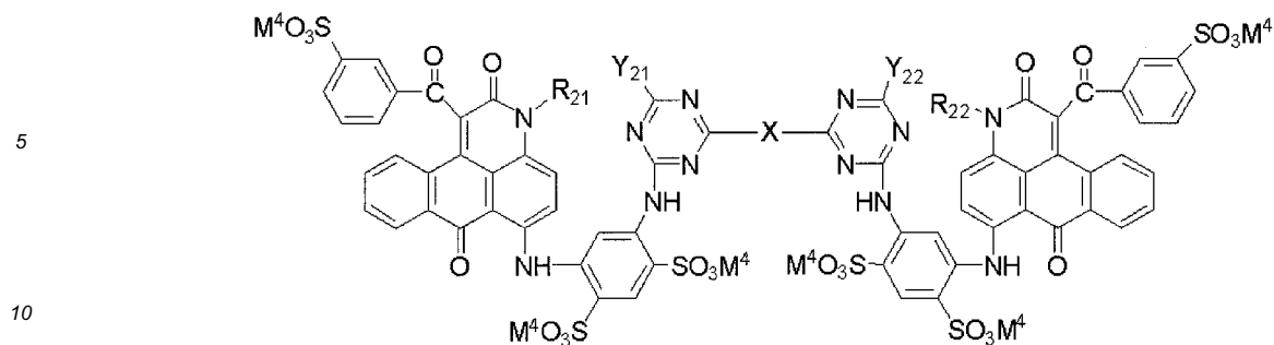
(B 4)
