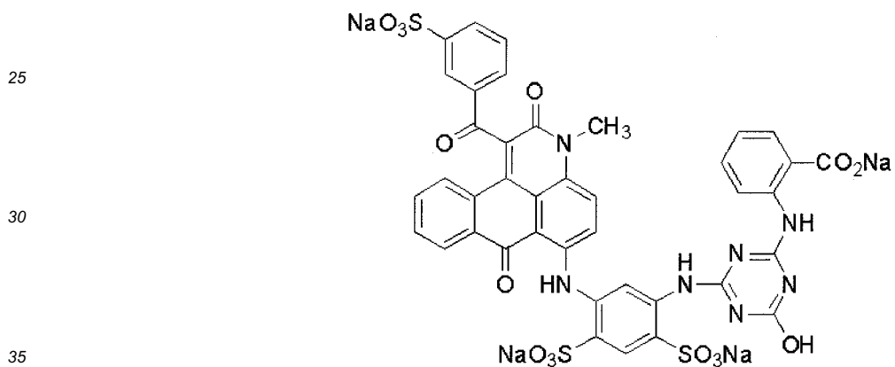
Compound (B3-2)
