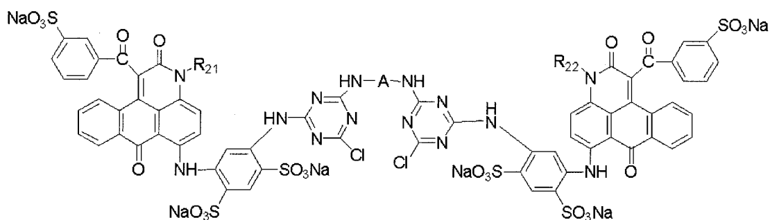
(B4-9)
