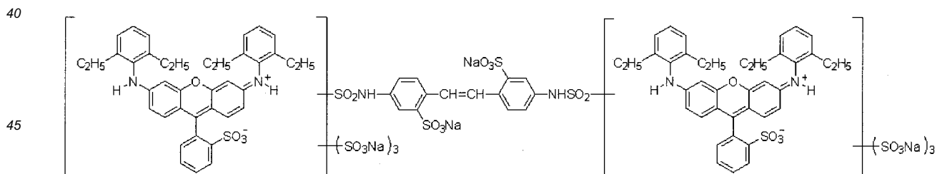
[0162] Compound B
