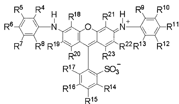
Formula (3)
