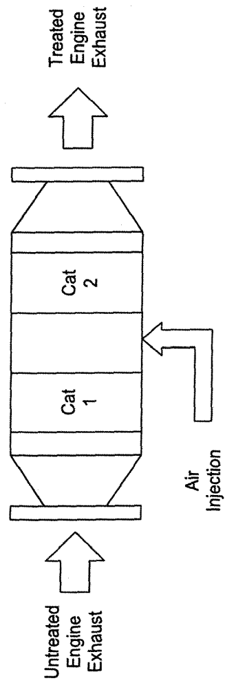
FIG. 3 (PRIOR ART)
