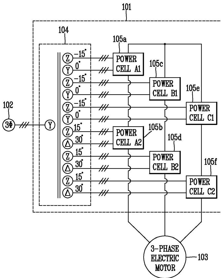
FIG. 1 RELATED ART
