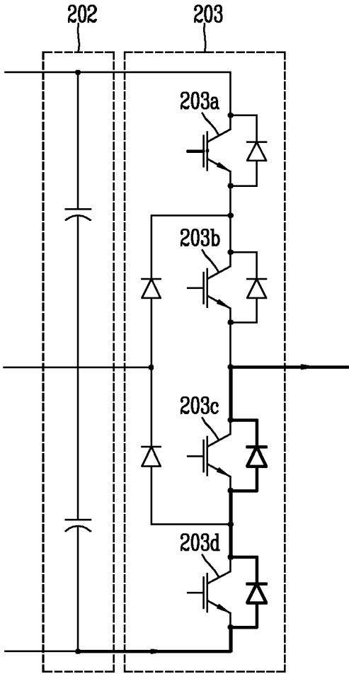
FIG. 3C RELATED ART
