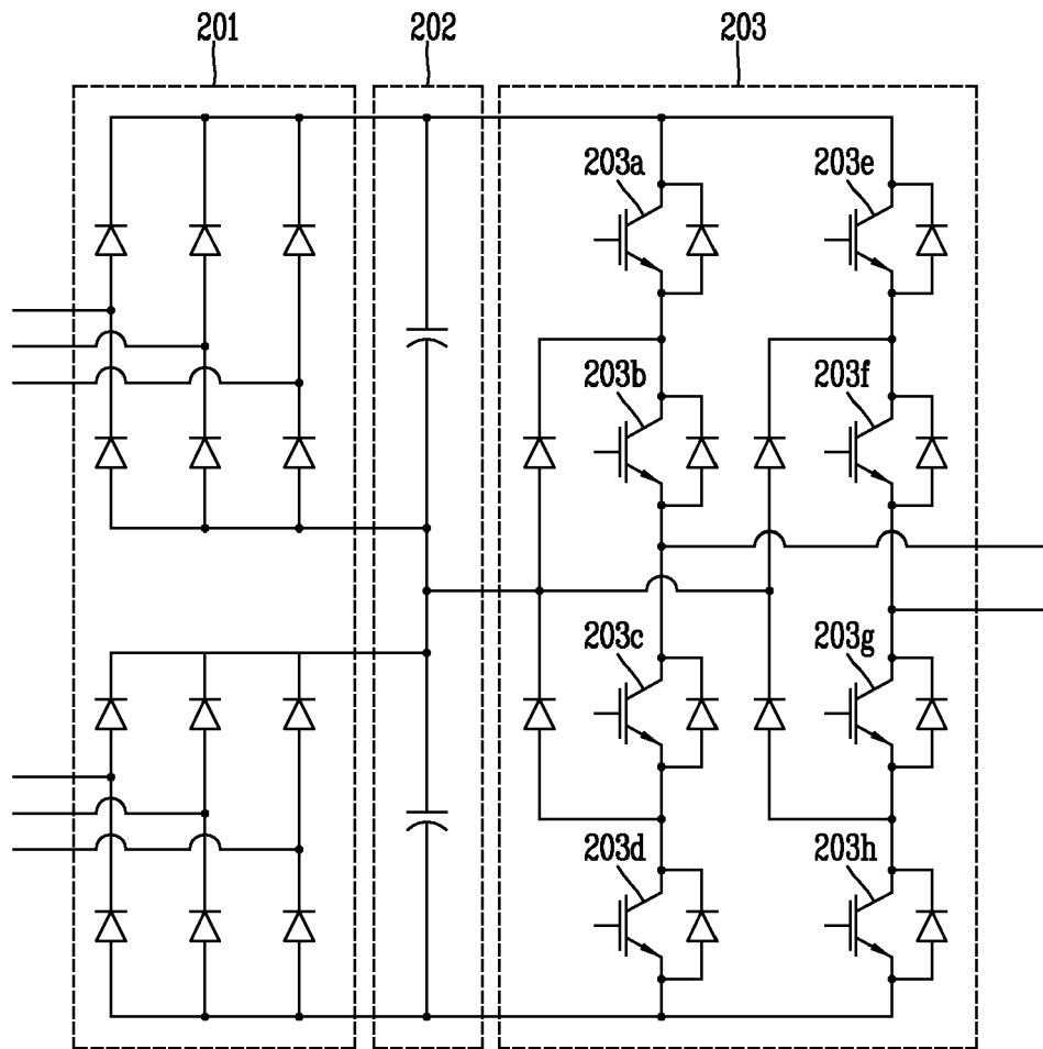
FIG. 2 RELATED ART
