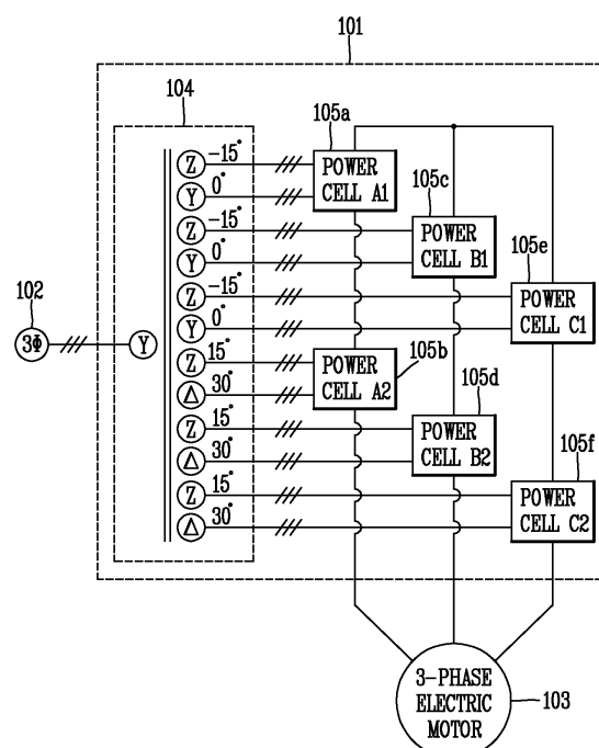
FIG. 1 RELATED ART
