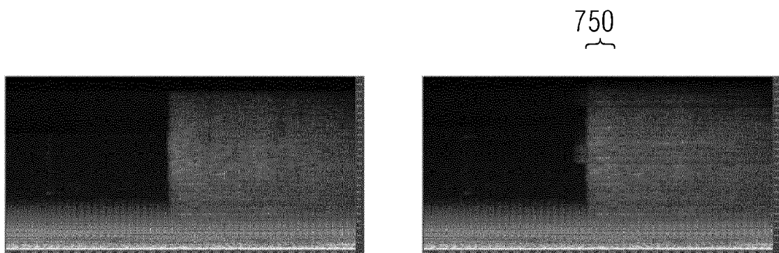
DFT spectrogram of the original signal (left panel); DFT spectrogram of the extended signal without TTS (right panel).
