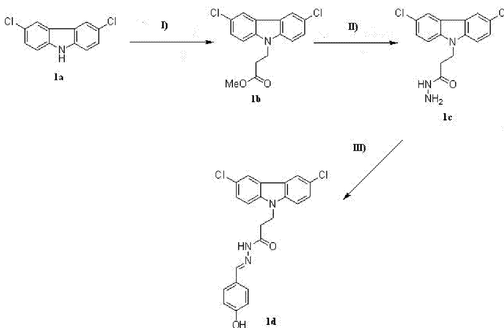
Synthesis scheme 3
