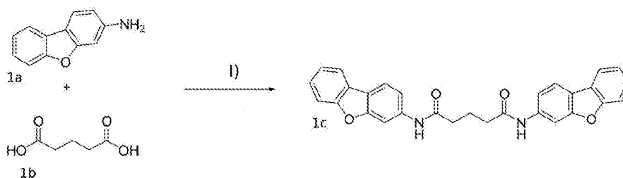
Synthesis scheme 4
