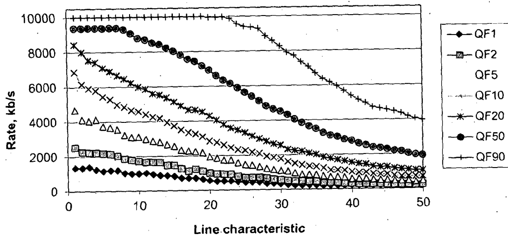
Equivalent quality curves from whole population quality plan for selected quality figures
