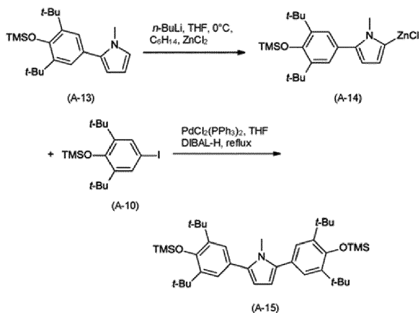
Reaction Formula (VII)
