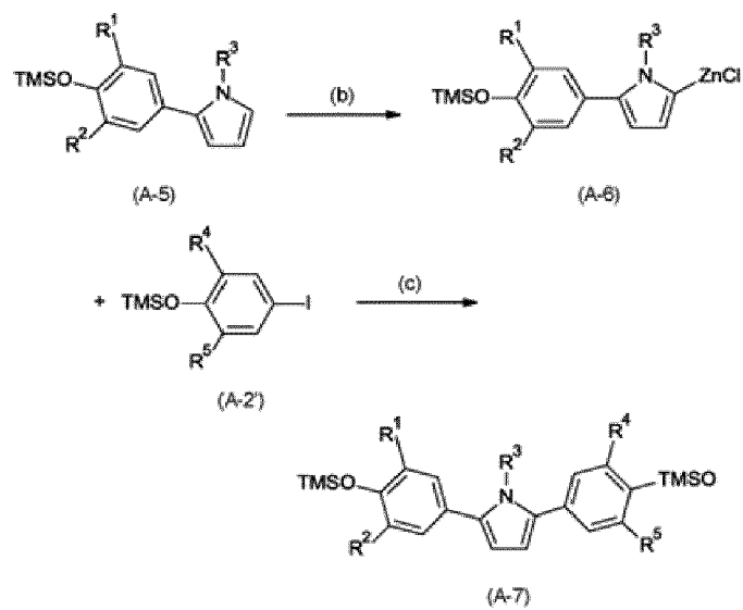
Reaction Formula (III)
