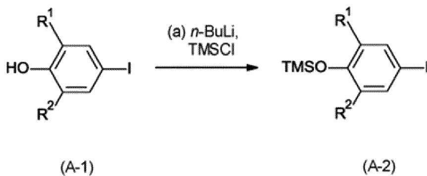
Reaction Formula (II)
