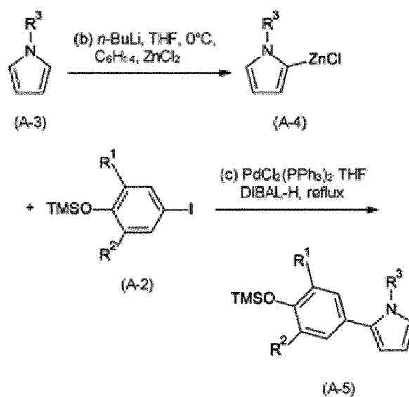
Reaction Formula (II)
