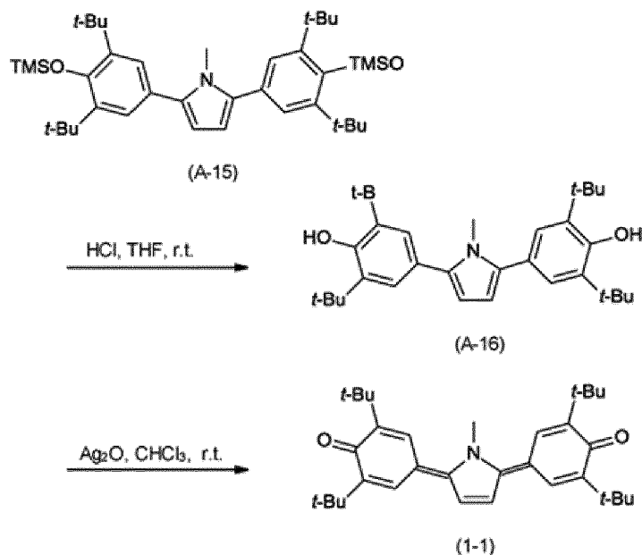
Reaction Formula (VIII)
