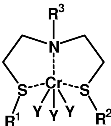
[Chemical Formula 1]
