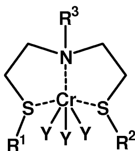
[Chemical Formula 1]
