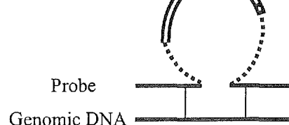
Mutant-type hybrid
