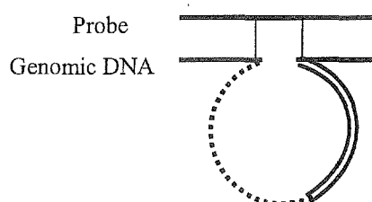
Mutant-type hybrid
