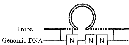
Wild-type hybrid
