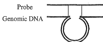
Wild-type hybrid
