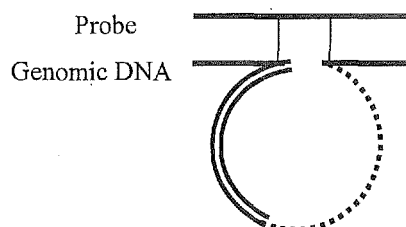
Mutant-type hybrid
