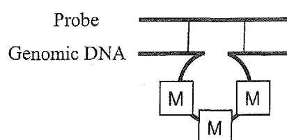
Wild-type hybrid
