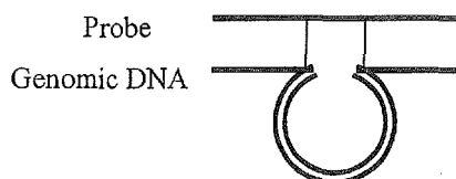
Wild-type hybrid
