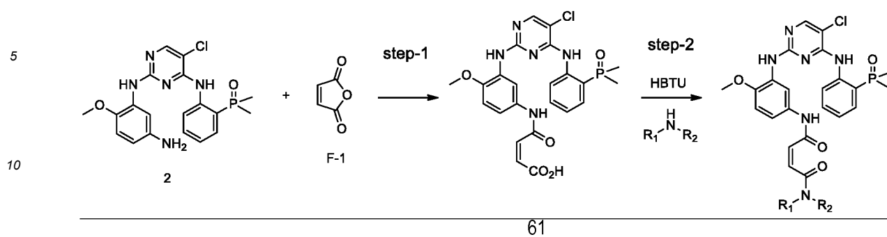
Scheme 31
