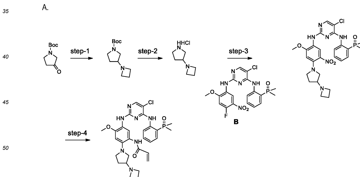
Scheme 37
