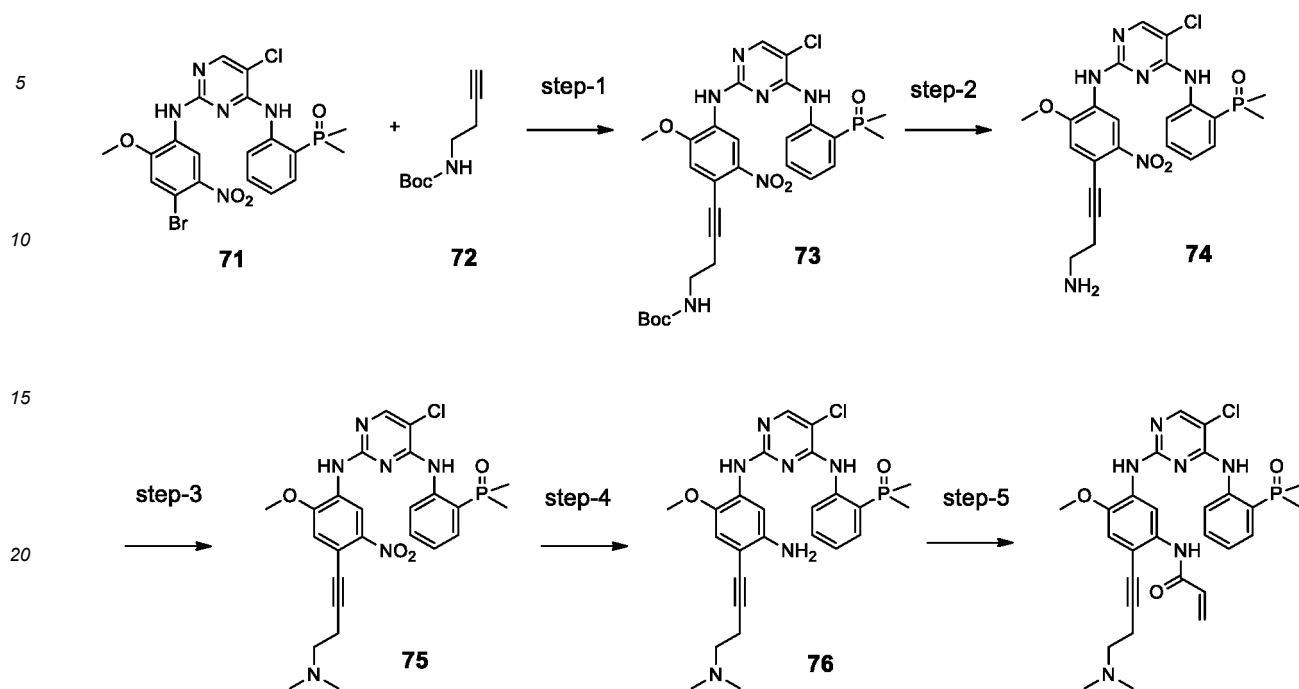
Scheme 42:
