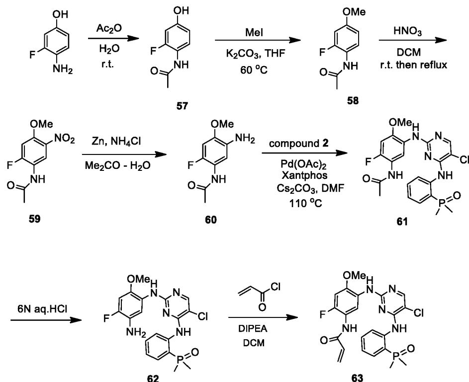
Scheme 22
