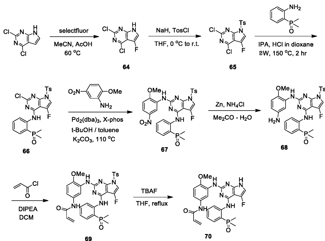
Scheme 23
