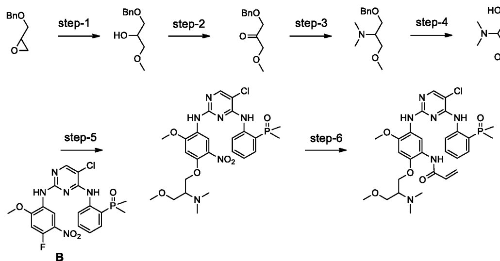
Scheme 34:
