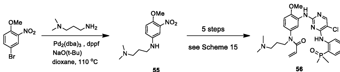
Scheme 21
