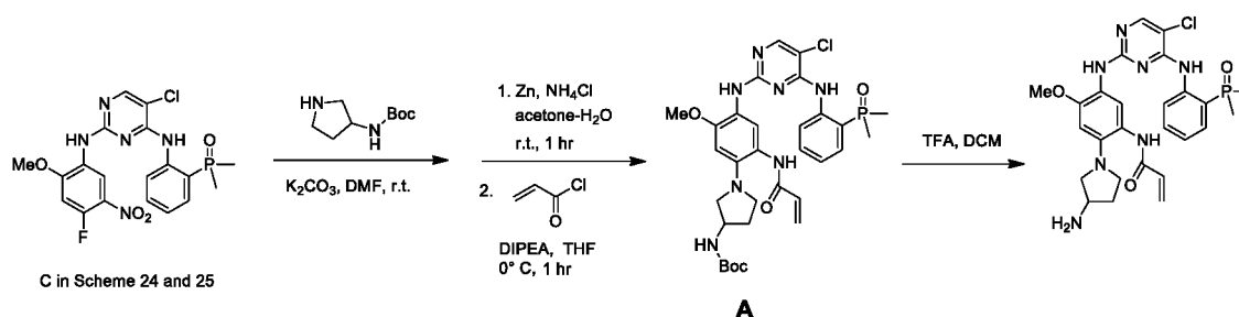
Scheme 30
