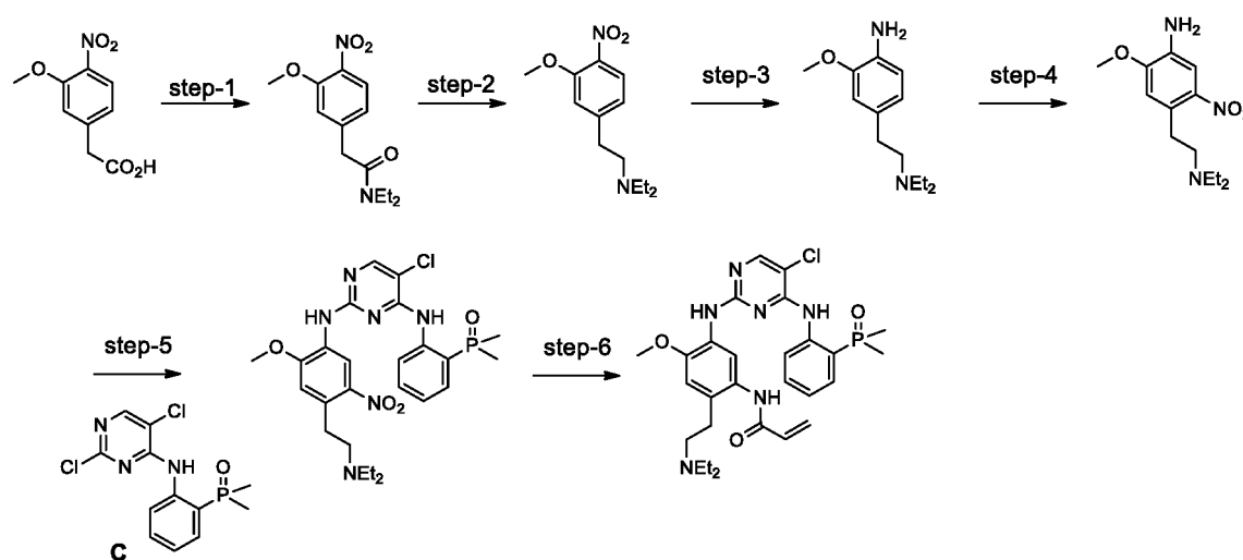
Scheme 40:
