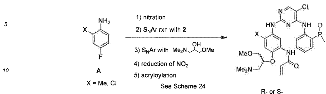
Scheme 47:
