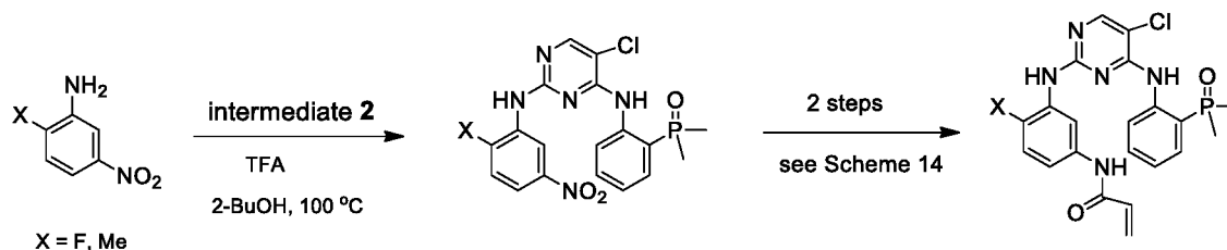
Scheme 28:
