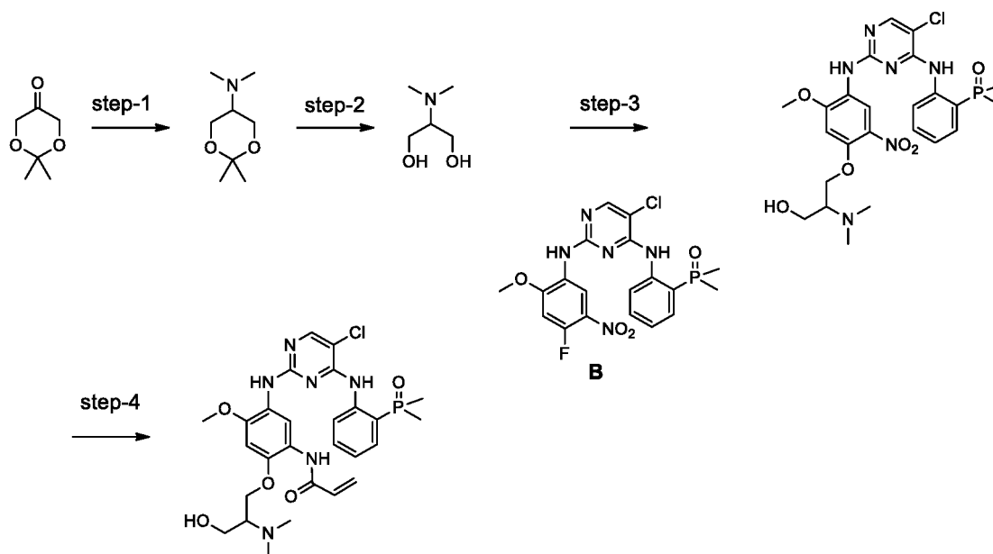
Scheme 33
