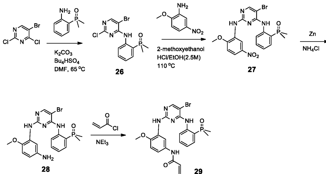
Scheme 12
