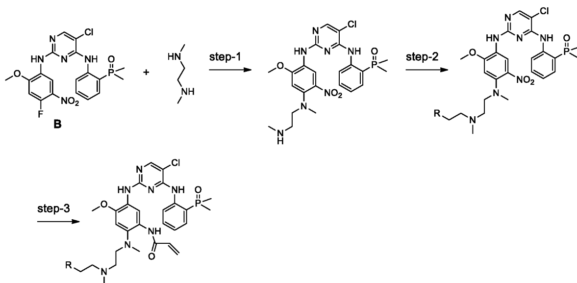
Scheme 35:
