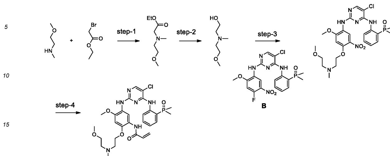
Scheme 36:
