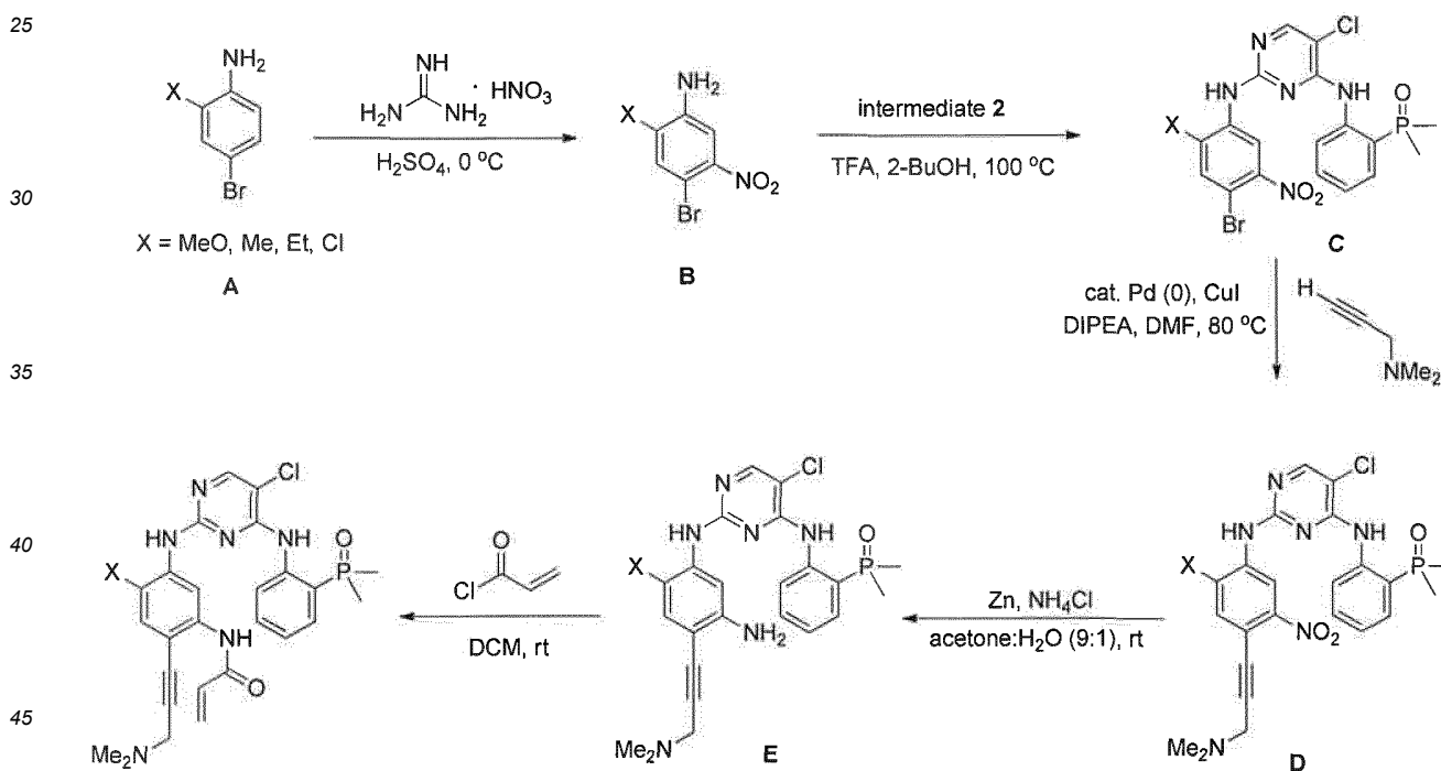
Scheme 48:
