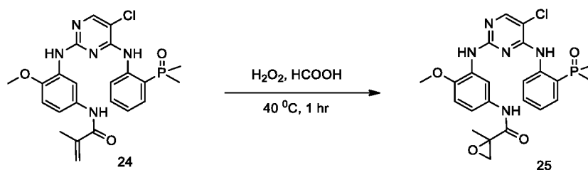
Scheme 10
