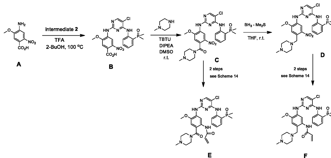
Scheme 29
