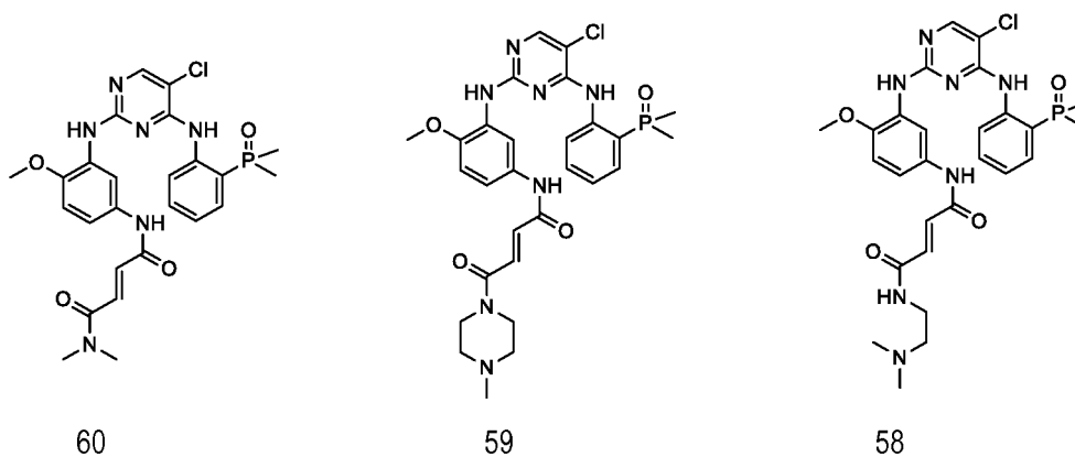
Scheme 32 : Example 65
