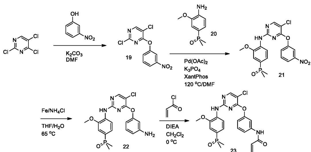
Scheme 9
