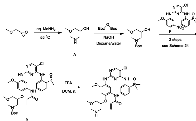
Scheme 41:
