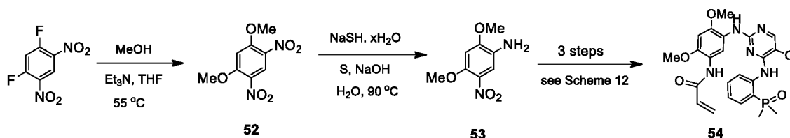
Scheme 20
