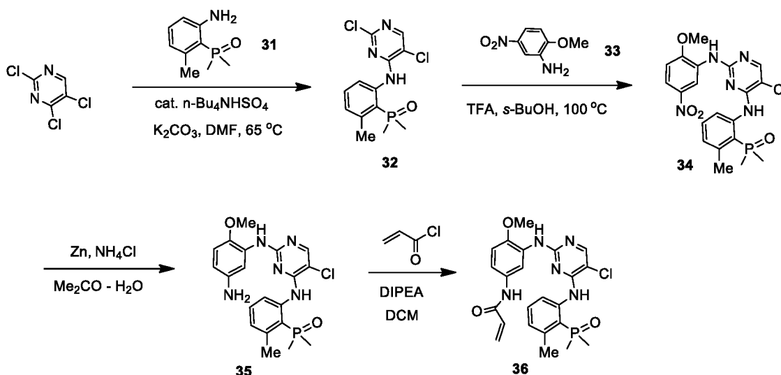
Scheme 14
