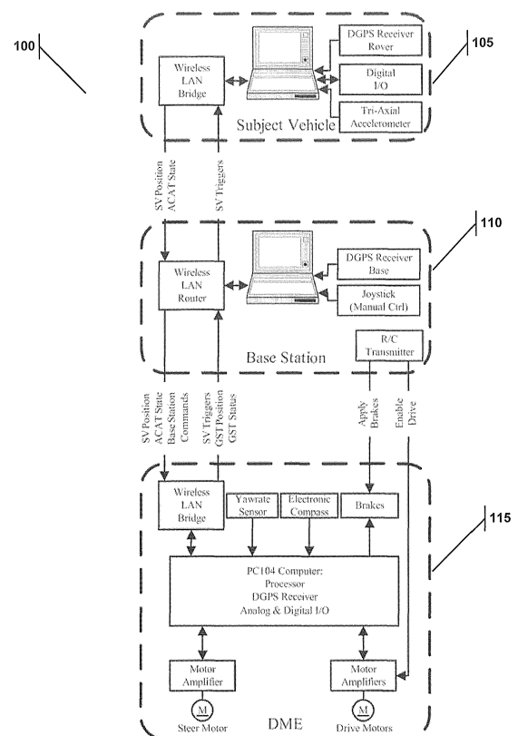
Example GST System Architecture FIG.1
