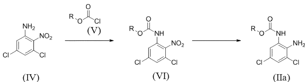
[Reaction Scheme 2]
