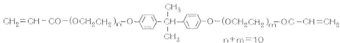
Chemical formula 5
