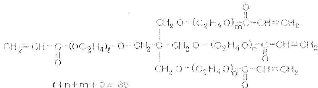
Chemical formula 7
